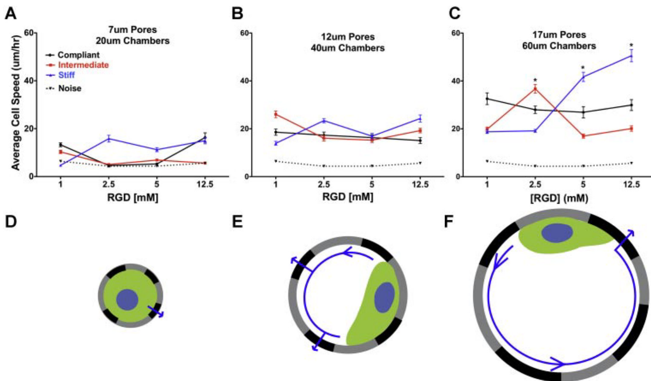
Figure 3. Changes in adhesivity and elastic moduli have the most pronounced impact on cell migration in the largest pore sizes. A and D : In the smallest pore diameter condition, cell speed is most often the same as the “noise” level, which is the speed of cells in the smallest void chambers that never migrate from their starting position. B and E : In the intermediate diameter pores, cell speed still appears to have minimal dependence on the levels of adhesion and stiffness; however, cell speed is qualitatively increased from the smallest pore size case, presumably due to room for intrachamber movement. C and F : In the largest pores, a dependence on adhesivity and elastic moduli emerges. The following points are statistically significant from all other data points: intermediate stiffness gel with 2.5 mM RGD, and stiff gels with 5 and 12.5 mM RGD ( P < 0.05 ).
