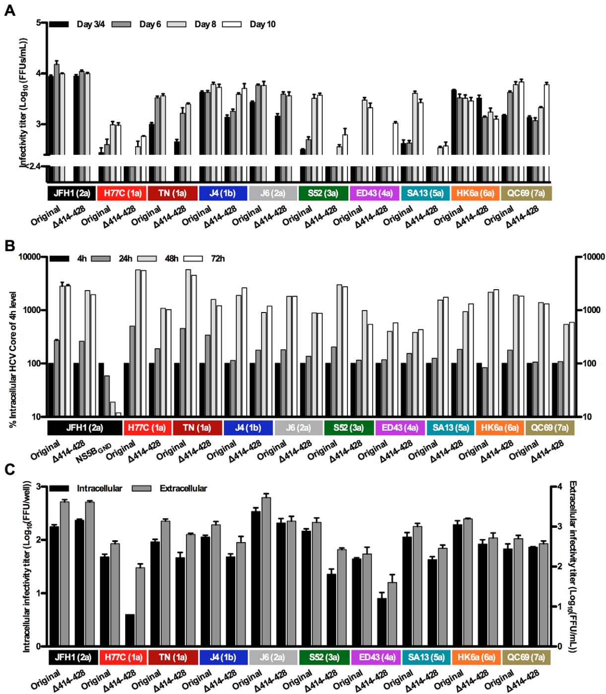
Figure 4. Infectivity titers and replication capacity of HCV NS5A domain III Δ414-428 mutants. (A) Infectivity titers in supernatant after transfection of Huh7.5 cells with original NS5A genotype recombinants and Δ414-428 mutants. The lower limit of detection in the experiments shown was 10 2.4 FFU/mL (indicated by the y-axis break). (B) As a measure of HCV RNA replication, S29 cells were transfected for 4 hours and intracellular HCV Core levels were measured after 4, 24, 48 and 72-hours. Values were normalized for transfection efficiency using 4-hour Core amounts of the respective recombinant. The JFH1(2a) NS5B GND mutant was included as a replication negative control. (C) Intra- and extracellular infectivity titers 48 hours after transfection of S29 cells. Intracellular titers are given per well of 4 × 10 5 transfected S29 cells. Colored boxes indicate the NS5A isolate and (genotype). Error bars indicate SEM of triplicate determinations, except for in (B) where JFH1(2a) was included in duplicates. doi:10.1371/journal.ppat.1002696.g004
