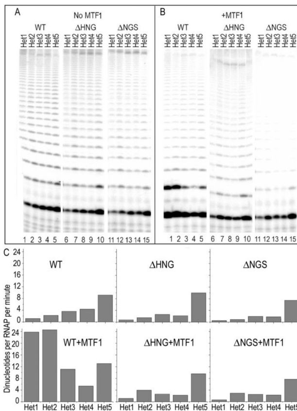
Figure 6. Deletion of scMtRNAP residues 631-633 or 632-634 affects dinucleotide synthesis as well as runoff transcription
