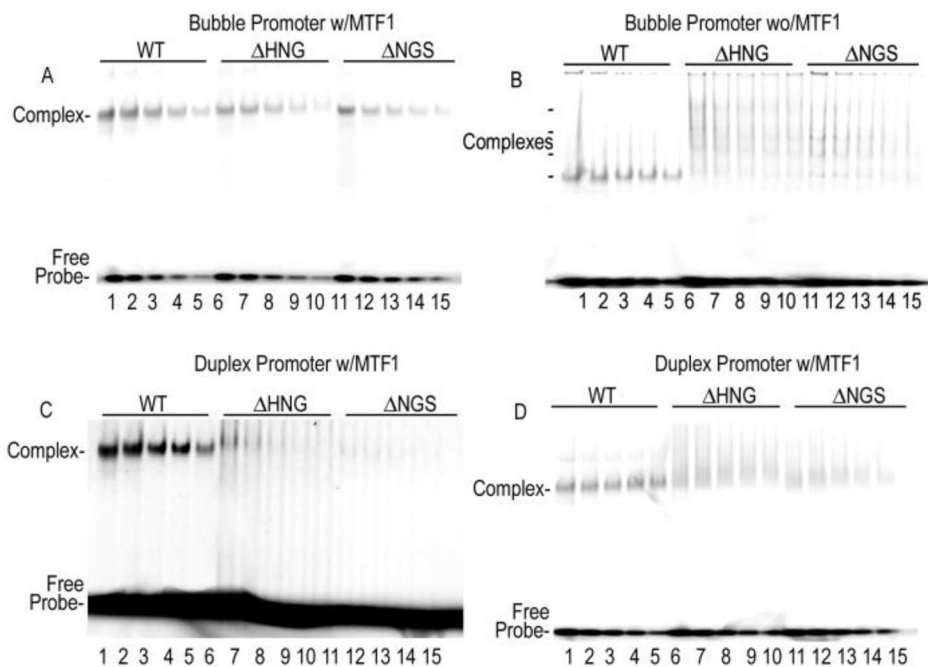
Figure 3. Quantitative EMSA reveals that \Delta HNG and \Delta NGS RNAPs bind bubble promoters with comparable affinity to WT RNAP, but bind duplex promoters more weakly A. Indicated RNAPs at 10^{-7} M were mixed with 10^{-7} M MTF1 and fluorescently labeled bubble promoter at concentrations that varied from 10^{-6} M (lanes 1, 6, 11) to 0.63 \times 10^{-7} M (lanes 5, 10, 15) in serial 2-fold dilutions and resolved on native 6% PAGE. B. As in A, but in the absence of MTF1. B. As in A, but without MTF1 present and with bubble promoter varied from 10^{-5} M (lanes 1, 6, 11) to 0.63 \times 10^{-6} M (lanes 5, 10, 15). C. As in A, but with duplex promoter varying from 4 \times 10^{-6} M (lanes 1, 6, 11) to 0.25 \times 10^{-6} M (lanes 5, 10, 15). D. As in C, but with RNAPs and MTF1 at 10^{-5} M and promoter varying from 10^{-4} M (lanes 1, 6, 11) to 0.63 \times 10^{-5} M (lanes 5, 10, 11). Note: In panels B and C, gels are shown over-exposed to allow visualization of the weak and/or multiple complex bands in the \Delta HNG/ \Delta NGS reactions.
