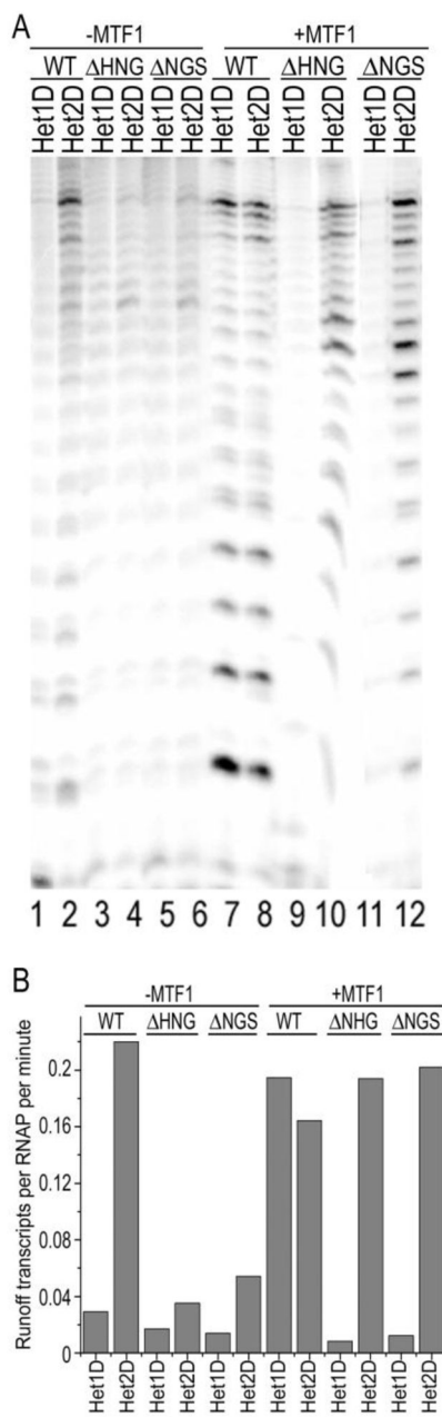
Figure 7. MTF1 and the intercalating hairpin make equal and synergistic contributions to transcription from promoters with mismatches at +1 and +2. A. Promoters containing mismatches at +2 (Het1D; odd numbered lanes) or +1 and +2 (Het 2D; even numbered lanes) transcribed with WT (lanes 1, 2, 7, 8), ΔHNG (lanes 3, 4, 9, 10) or ΔNGS (lanes 5, 6, 11, 12) MtrRNAPs in either the absence (lanes 1–6) or presence (lanes 7–8) of MTF1. B: Rates of runoff transcription on the indicated promoters and by the indicated MtrRNAPs with or without MTF1.
