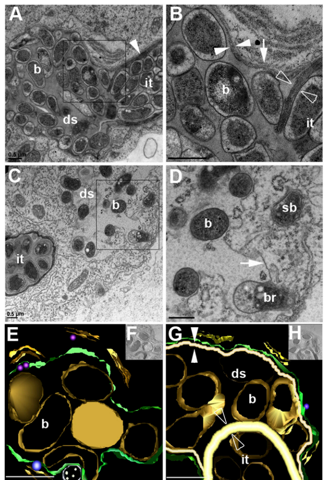
Fig. 2. MtVAMP721d and MtVAMP721e are essential for the formation of unwalled infection droplets at infection threads. (A and B) EM images of an infection thread in a 35S::RNAiVAMP721d:VAMP721e nodule (A) and magnification of the designated area (B). The infection thread (it) is filled with bacteria and bound by a cell wall (arrowhead). At the tip of the thread a droplet-like structure (ds) filled with bacteria (b) is formed. The droplet-like structure is surrounded by a membrane (B, arrow) extending from the infection thread plasma membrane and bound by a cell wall (B, white opposed arrowheads) that is markedly thinner than the wall around the infection thread (B, open opposed arrowheads). (C and D) EM images of an infection thread in a control nodule (C) and magnification of the designated area (D). The unwalled droplet (ds) is bound by a membrane (arrow), but a cell wall is absent. Bacteria (b) are being released (br) and form symbiosomes (sb). (E–H) Electron microscopy computed tomography and 3D reconstruction of an infection thread in a control (E and F) and 35S::RNAiVAMP721d:VAMP721e (G and H) nodule. Analyses were performed on 360-nm-thick sections. In the droplet structure (ds) of RNAiVAMP721d:VAMP721e nodules (G and H) the bacteria are separated from the host membrane (green) by a cell wall (white, opposed arrowhead). This cell wall is markedly (~3 \times ) thinner (white opposed arrowheads) than the cell wall of the infection thread (it) at which a droplet structure is formed (open opposed arrowheads). The unwalled droplets in nodules on control roots (E and F) are bound only by the host membrane (green), which allows the bacteria (b, gold) to come into close contact with it. (Scale bars, 0.5 \mu m in A–G.)
