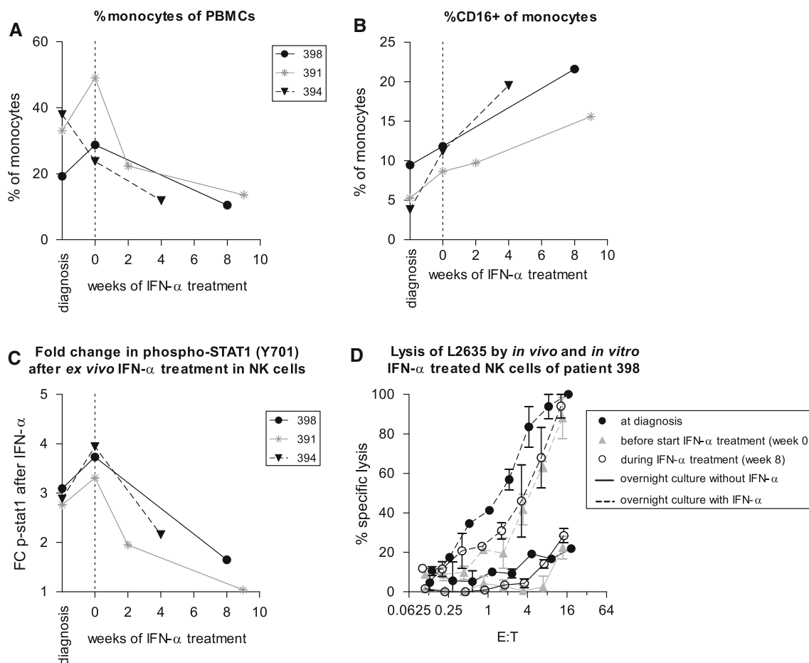
Fig. 2 Effect of in vivo IFN- \alpha administration on monocytes and NK cells. a Following in vivo treatment with IFN- \alpha of three osteosarcoma patients, the percentage of monocytes of PBMCs decreased. b The relative percentage of CD16-positive monocytes increased. c NK cells which had been exposed to IFN- \alpha in vivo showed less phosphorylation of STAT1 in response to ex vivo IFN- \alpha stimulation. d Cytolysis of the autologous osteosarcoma target cell line L2635 by PBMCs of
