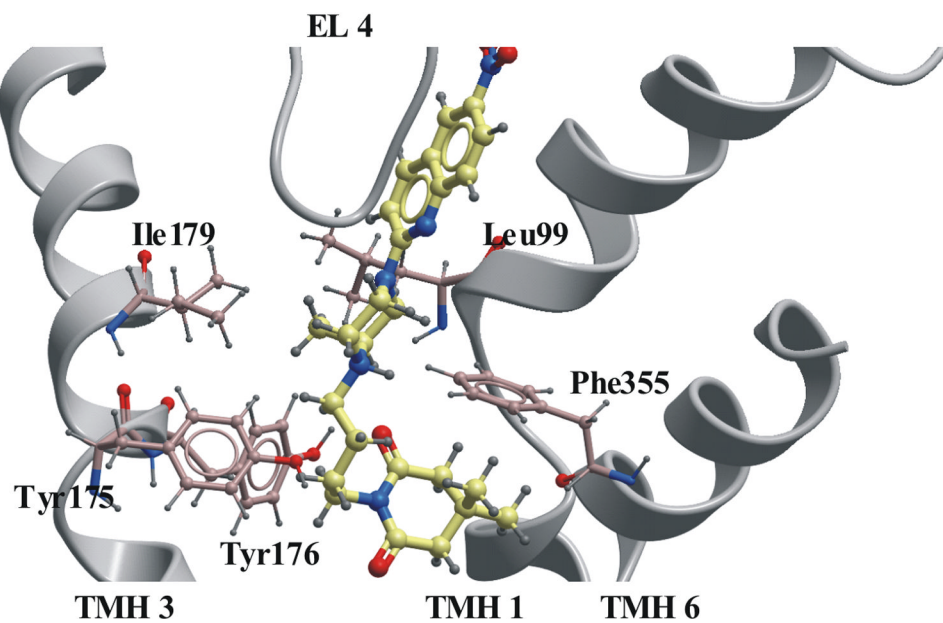
Fig. 9. The interactions between methyl group at the piperazine ring of buspirone analogues with SERT model in the outward-facing conformation: (a) ligand 12 (b) ligand 18 .
