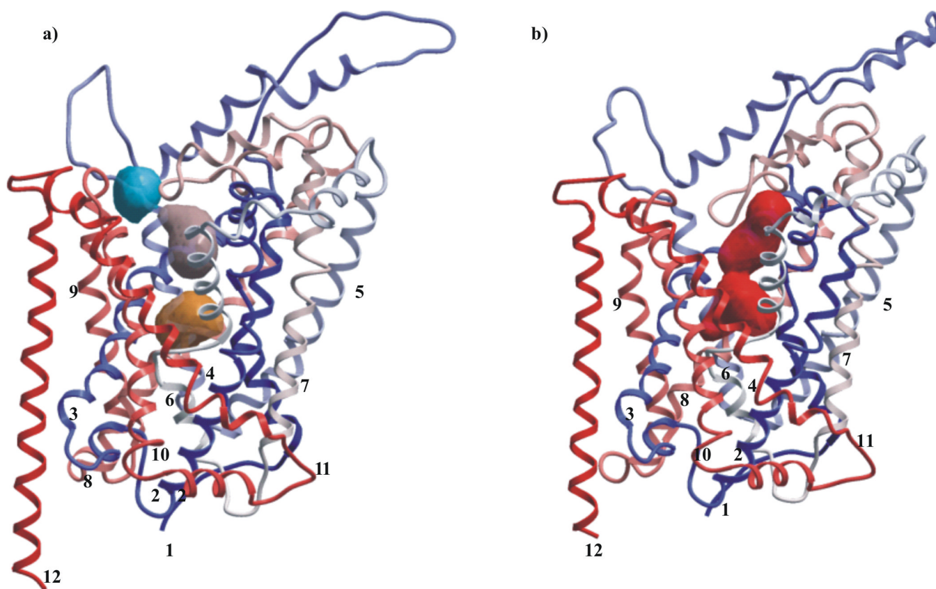
Fig. 5. Serotonin transporter (SERT) models based on the X-ray structure of the LeuT Aa from Aquifex aeolicus : (a) the substrate-occluded conformation, (b) the outward-facing conformation. The models are coloured from amino (red) to carboxy (blue) terminal. Binding pockets identified by using ICM PocketFinder: putative binding pocket is displayed in orange color, vestibular binding pocket, consisting of the two subpockets, is displayed in a blue and pink color. The large binding pocket of SERT in the outward-facing conformation is displayed in red color.
