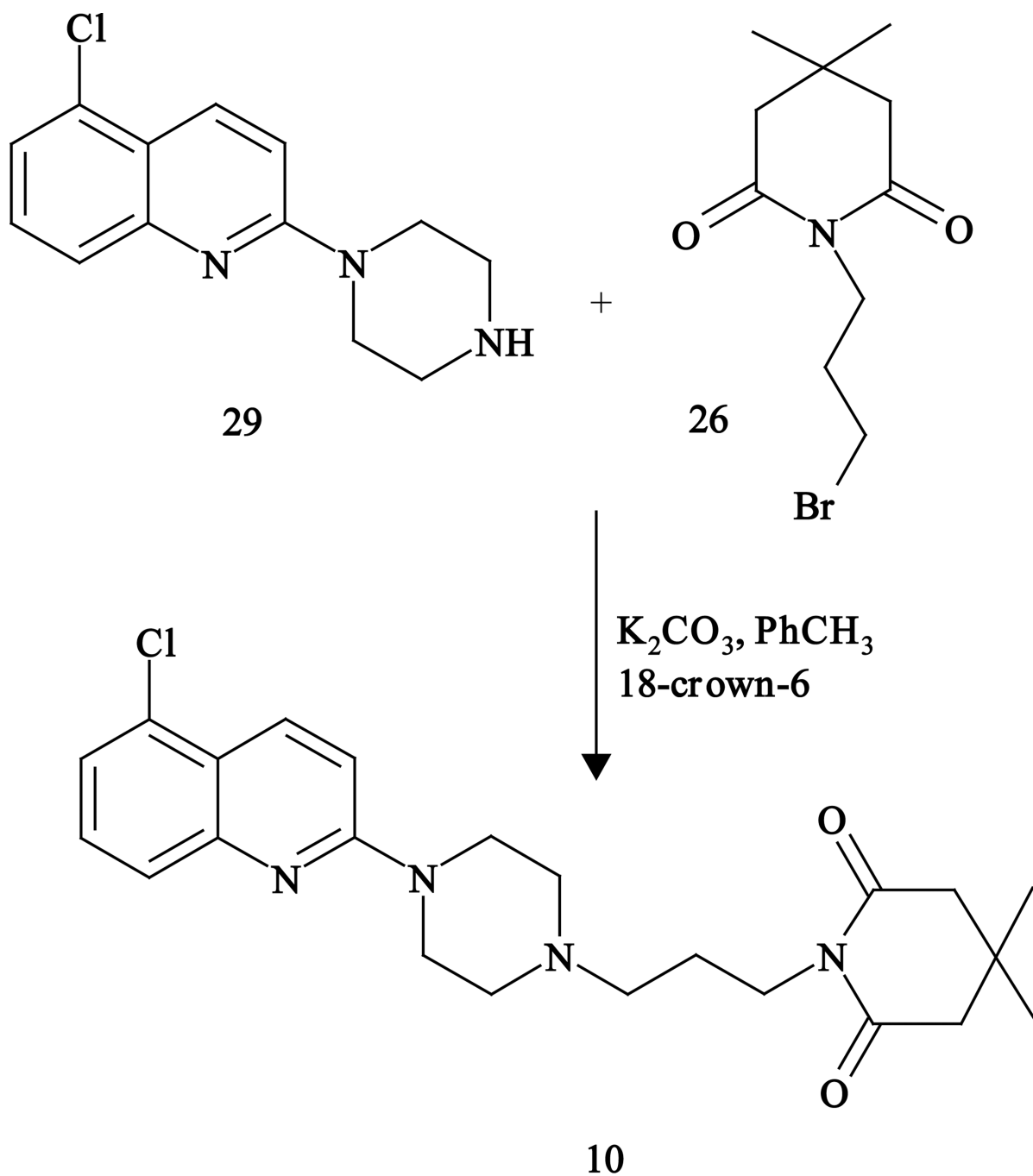
Fig. 3. Synthesis of 5-chloro derivative 10 .
