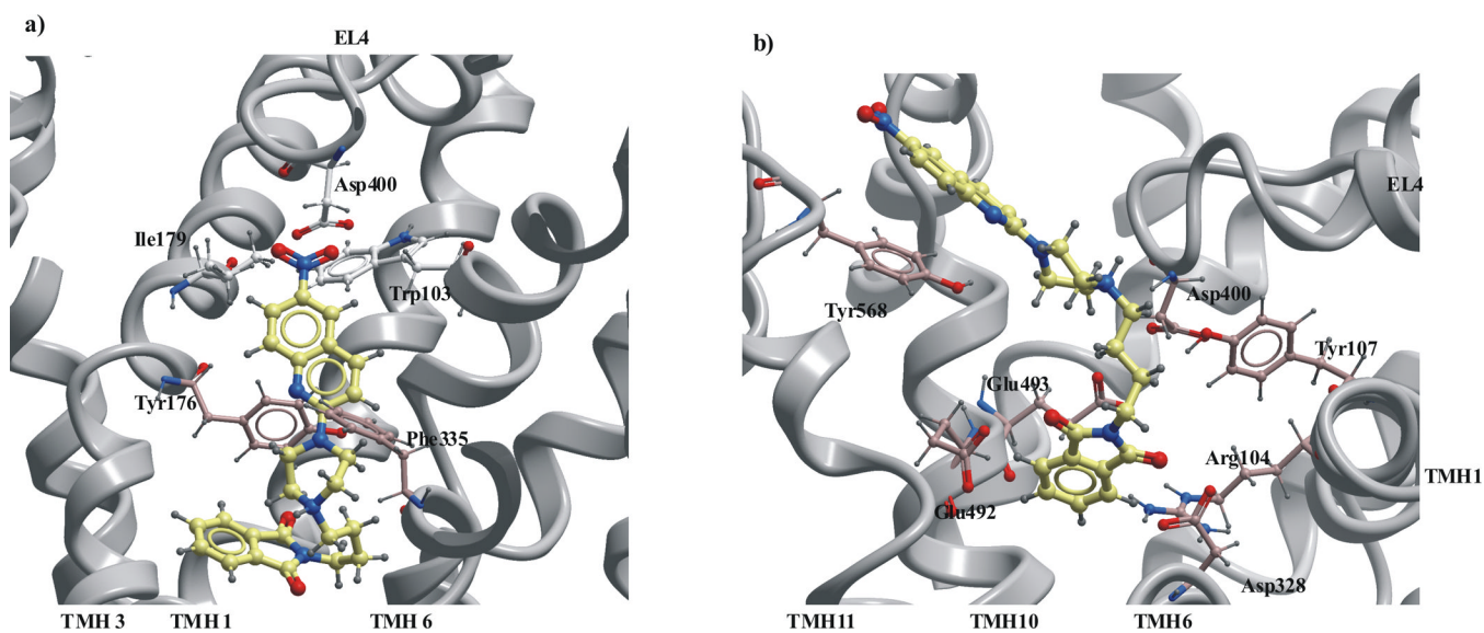
Fig. 6. The docking of nitroquipazine derivatives to the a) putative binding site, b) vestibular binding site of the SERT model in the closed conformation.
