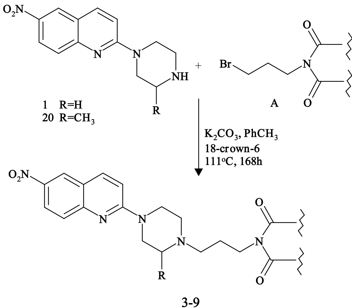
Fig. 1. General scheme of the preparation of 6-nitroquipazine buspirone analogues 3-9.
