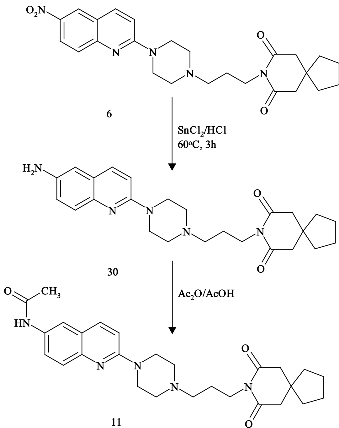
Fig. 4. Synthesis of 6-amido derivative 11 .
