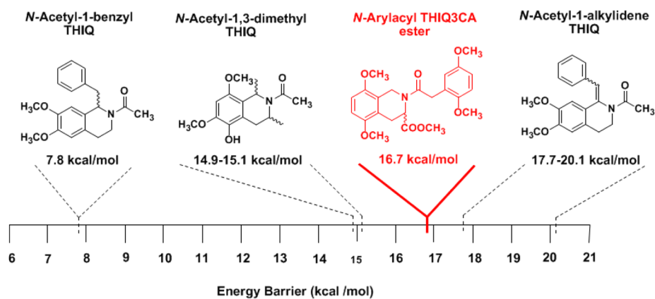
Figure 5. THIQ derivatives display a wide range of energy barriers for conformational transitions. The N -arylacyl THIQ3CA esters studied in this work show a distinct high energy barrier of ~17 kcal/mol.
