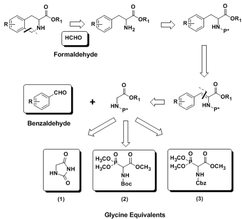
Figure 1. Retrosynthetic analysis for the synthesis of THIQ3CA scaffold using glycine equivalents.
