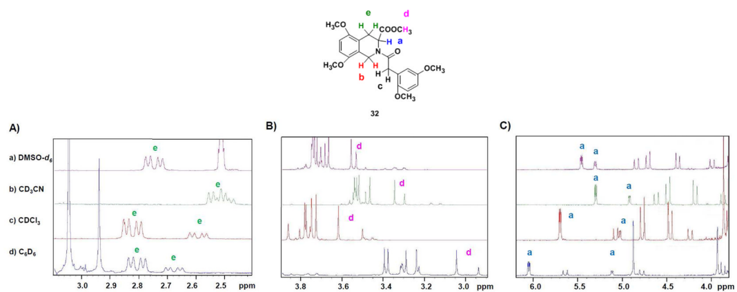
Figure 3. Solvent-dependent changes in the conformational isomerism of 32 . A) 3.1-2.4 \delta ; B) 3.9-2.8 \delta ; and C) 6.2-3.8 \delta
