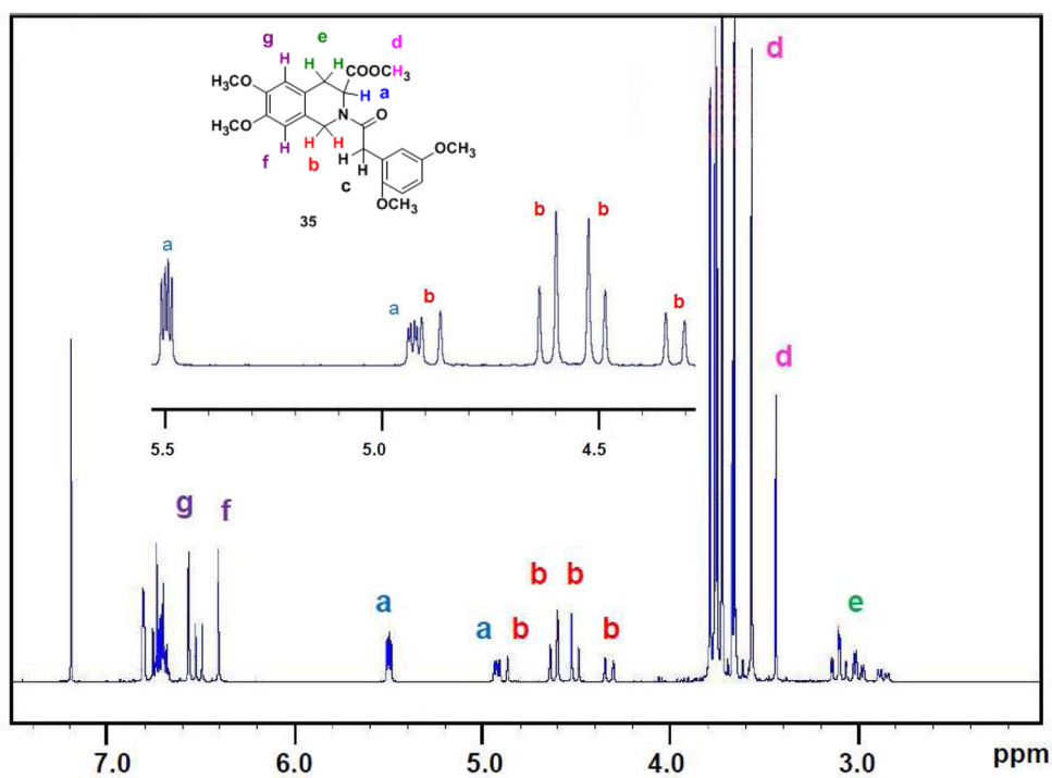
Figure 2. ^1\text{H} NMR spectrum of THIQ3CA analog 35 in \text{CDCl}_3 showing duplicity of signals at ambient temperature. Inset shows 6.0-4.0 \delta region, assignable to 'a' and 'b' protons, for better clarity.
