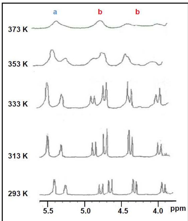
Figure 4. Temperature effect on the conformational isomerism of 32 in DMSO- d 6 . The entire 1 H NMR spectrum of 32 was recorded but only the 5.6-3.8 δ range is shown for enhanced clarity. 1 H NMR spectra at 293, 313, 333 and 353 K were recorded on a Varian 300 MHz instrument, while the spectrum at 373 K was recorded on a Bruker 400 MHz.
