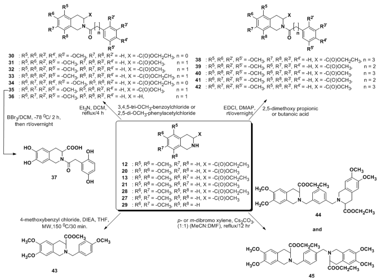
Scheme 3. Synthesis of N -substituted THIQ3CA-based library.
