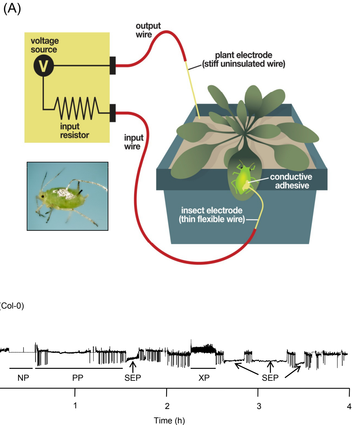
Figure 2. Electrical penetration graph (EPG) setup used for characterizing the feeding behavior of aphids on its host plant.
