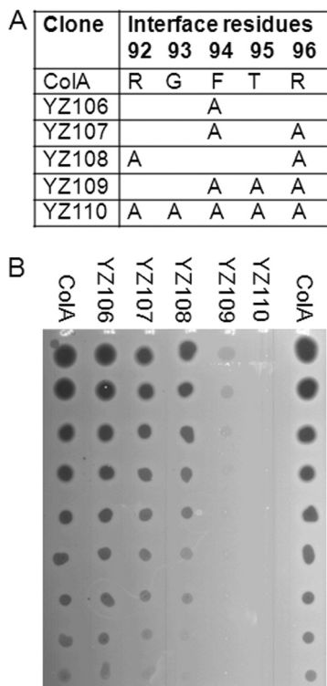
FIGURE 3. Effects of TolA box mutations of ColA on activity of ColA are cumulative. A, individual (pYZ106), double (pYZ107 and pYZ108), and multiple mutations of the TolA box of ColA (pYZ109 and pYZ110) were engineered using PCR mutagenesis, and the mutant polypeptides were purified and spotted onto a lawn of sensitive E. coli cells. B, zones of clearing indicative of cell killing were reduced in mutants containing successively more mutations and disappeared in all mutants containing three or more mutations.
