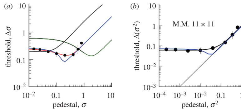
Figure 3. The results (filled circles) for observer MM in the 11 \times 11 grid condition, and the fits of various models described more fully in the text. (a) The data as a function of the standard deviation of the uniform distribution from which the dot positions were sampled, in units of the canonical dot spacing. The red curve passing through all the data points is the best fit of the undersampling model, with six dots per sample. The blue curve is a fit of the sensory threshold model with the threshold constrained to be the same as the variance of the internal noise. The green curve is the best fit of the undersampling model with the number of samples constrained to be the total number of dots ( 11 \times 11 ). The black curve with no dip is the fit of the undersampling model with n = 2 . (b) Thresholds ( \sigma^2 ) as a function of pedestal ( \sigma^2 ). The black curve is the best fit of the undersampling model. The blue curve is a fit of the sensory threshold model with the threshold constrained to be the same as the variance of the internal noise.
