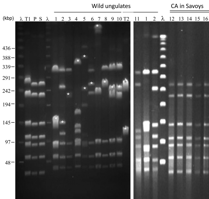
FIG 3 Representative PFGE patterns of M. agalactiae isolates following digestion of their chromosomal DNA by MluI. Lanes 1 to 11, M. agalactiae strains from wild fauna (strains 13387, 14628, 14797, 15009, 15044, 15196, 15261, 15406, 15341, 15379, and 13501, respectively, with lanes 1 and 2 represented twice). For history, see Table 1 . Lane T1, M. agalactiae PG2; lane T2, M. agalactiae 5632; lane P, strain 4206, used as representative of the clonal population currently circulating in the Pyrénées-Atlantiques region. Lanes 12 to 16 represent several isolates collected in Savoy from domestic small ruminants during the historical episode of CA. Strain 4908 (lane S) was chosen as a representative. Stars indicate fragments that were detected by Southern blotting with a probe targeting an ICE (CDS22) of M. agalactiae strain 5632. Lane λ contained lambda DNA concatemers for which the molecular sizes are indicated on the right.
