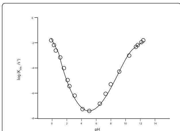
Figure 1 The RNA phosphodiester bond is most stable at pH 4-5 at 90°C. Hydrolysis of the dinucleoside 3',5'-UpU at 90°C as a function of pH. Figure reprinted with permission from [15] Oivanen et al. ©1998 American Chemical Society; data used with permission from [10] Järvinen et al. ©1991 American Chemical Society.
