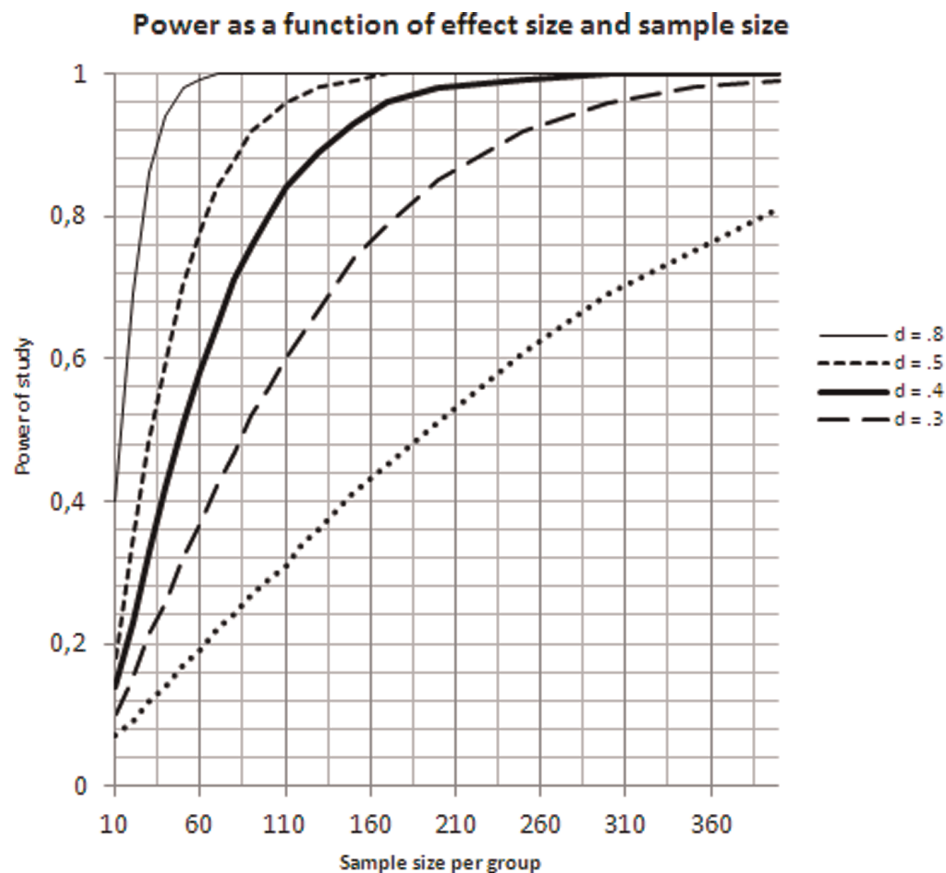
Figure 1. Power of study as a function of sample size. This figure shows the power of a study with two independent groups as a function of sample size for different levels of effect size (assuming that alpha, 2-tailed, is set at .05). For a small effect size ( d = .2 ) we would need two samples of 393 participants to yield a power of 80%. This means that there is 80% chance of finding a significant difference between the groups, given that an effect of this size exists at the population level. For a medium effect size ( d = .5 ) we would need two samples of 64 participants to achieve this level of power. For a large effect size ( d = .8 ) we need 26 participants per group. doi:10.1371/journal.pone.0038081.g001
