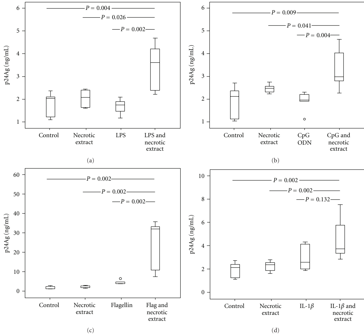
FIGURE 2: Necrotic extract and TLR-ligands in complexes upregulate viral replication in U1 cells. U1 cell cultures were stimulated with necrotic extract (HMGB1 concentration 1 \mu g/mL) and Toll-like receptor ligands: LPS 10 ng/mL (a), CpG-ODN 1 \mu g/mL (b), flagellin 50 ng/mL (c), and IL-1 \beta 0.25 \mu g/mL (d) alone or in complexes. Supernatants from mock cells served as controls. Supernatants were collected from cell cultures after 72 hours. Results from three independent experiments in duplicates are presented.
