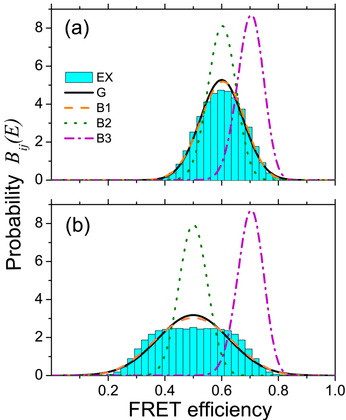
Figure 3. Comparison of various approximations for the probability of FRET efficiency, B_{ij}(E) , in the bins that undergo a single j \rightarrow i transition. The exact (EX) histograms (bars) are calculated using Eq. (21). They are compared with the Gaussian (G) distribution (solid line, Eqs. (33)–(35)) and with Beta distributions, Eq. (36), with three different sets of parameters: parameters B1 result in the correct mean and variance (dashed line, Eq. (37)), B2 are determined by the average count rates (dotted, Eq. (38)), and B3 by the count rates of the initial state (dashed-dotted, Eq. (39)). Mean number of donor and acceptor photons in a bin is nT = 100 , FRET efficiencies of the states are (a) \xi_i = 0.5 , \xi_j = 0.7 ; (b) \xi_i = 0.3 , \xi_j = 0.7
