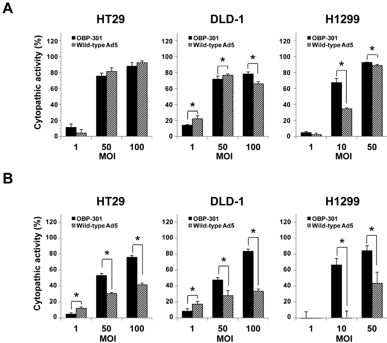
Figure 3. Cytopathic effect of OBP-301 and wild-type adenovirus serotype 5 (Ad5) under normoxic or hypoxic conditions. Cells were infected with OBP-301 (solid bars) or wild-type Ad5 (diagonal bars) at the indicated MOIs under normoxic (A) or hypoxic (B) conditions for 3 days. Cell viability was determined using an XTT assay. Cell viability was calculated relative to that of mock-treated cells, whose viability was set at 100%. Cytopathic activity was further calculated using the following formula; Cytopathic activity (%) = 100 (%) – cell viability (%). The results shown are the mean values \pm SD of quadruplicate experiments. Statistical significance (*) was determined as P < 0.05 (Student's t test). doi:10.1371/journal.pone.0039292.g003
