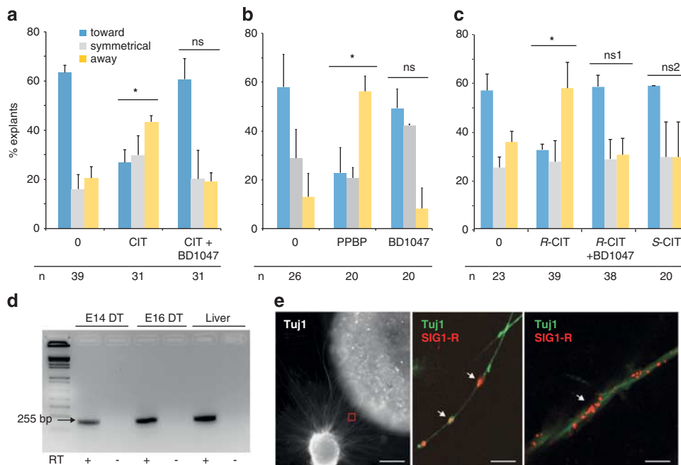
Figure 3 The effect of ( RS )-CIT is mediated by the \sigma 1 receptor. (a) ( RS )-CIT (CIT, 10 \mu\text{M} ) significantly alters the response of wild-type thalamic axons to netrin-1. The effect is blocked by co-incubation with the \sigma 1 antagonist BD-1047 (CIT + BD-1047; CIT, 10 \mu\text{M} ; BD-1047, 1 \mu\text{M} ; *, \chi^2 = 26.22 , P < 0.0001 , df = 2 ; \chi^2 ; ns, not significant, \chi^2 = 0.57 , P = 0.7495 , df = 2 ; \chi^2 ). (b) BD-1047 alone has no effect, but the \sigma 1 agonist PPBP ( 1 \mu\text{M} ) switches the response of thalamic axons to netrin-1, similar to the effect of citalopram (*, \chi^2 = 43.20 , P < 0.0001 , df = 2 ; \chi^2 ; ns, not significant, \chi^2 = 4.16 , P = 0.1247 , df = 2 ; \chi^2 ). (c) ( R )-CIT (R-CIT, 10 \mu\text{M} ), but not ( S )-CIT ( 10 \mu\text{M} ), significantly alters the response of thalamic axons to netrin-1. The effect is blocked by co-incubation with the \sigma 1 antagonist BD-1047 (R-CIT + BD-1047; R-CIT, 10 \mu\text{M} ; BD-1047, 1 \mu\text{M} ; *, \chi^2 = 9.85 , P = 0.0072 , df = 2 ; \chi^2 ; ns1, not significant, \chi^2 = 0.41 , P = 0.8132 , df = 2 ; \chi^2 ; ns2, not significant, \chi^2 = 0.68 , P = 0.7093 , df = 2 ; \chi^2 ). n indicates the number of explants tested in each condition. (d) PCR amplification of dorsal thalamus cDNA shows that \sigma 1 is expressed in the structure at E14 (E14 DT) and E16 (E16 DT); cDNA from the adult liver was used as a positive control for the reaction (liver). RT +/- indicates the presence (+) or absence (-) of reverse transcriptase during the cDNA synthesis reaction. (e) The \sigma 1 receptor protein is expressed along thalamic axons growing in vitro . Immunostaining was performed on thalamic explants (E14) grown in vitro for 3 days in apposition to HEK cells expressing netrin-1 (left panel). Right panel is a high magnification of the boxed area on the left panel. White arrows point to varicose-like structures showing intense \sigma 1 labeling. Scale bars = 400 \mu\text{m} (left panel), 10 and 5 \mu\text{m} (right panels, respectively).
