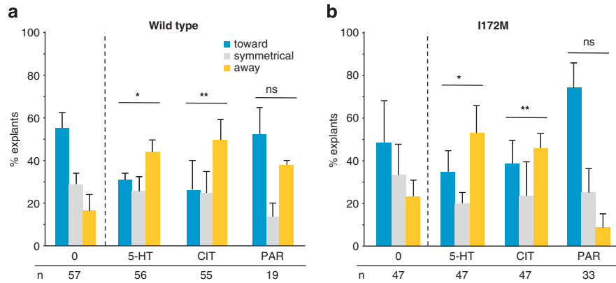
Figure 2 Effect of ( RS )-CIT in thalamic explants from wild-type and SERT M172 mice. (a) 5-hydroxytryptamine (5-HT) ( 30 \mu\text{M} ) or ( RS )-CIT (CIT, 10 \mu\text{M} ) significantly affect the response of wild-type thalamic axons to netrin-1 (*, \chi^2 = 20.06 ; **, \chi^2 = 27.43 , P < 0.0001 , df = 2 ; \chi^2 ). The effect remains in cultures from SERT M172 (b) embryos, where ( RS )-CIT affinity for SERT is decreased ( \sim 1000 fold) compared with wild-type (*, \chi^2 = 21.86 ; **, \chi^2 = 18.90 , P < 0.0001 , df = 2 ; \chi^2 ; ns, not significant, \chi^2 = 5.2 , P = 0.0743 , df = 2 ; \chi^2 ). In both cultures, the SSRI paroxetine (PAR, 10 \mu\text{M} ) has no significant effect. n, number of explants tested in each condition.
