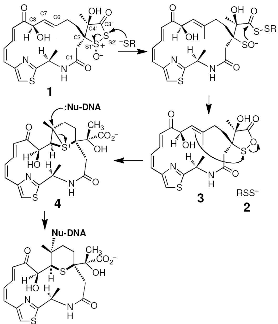
Scheme 1. Thiol-activated DNA alkylation by leinamycin.
