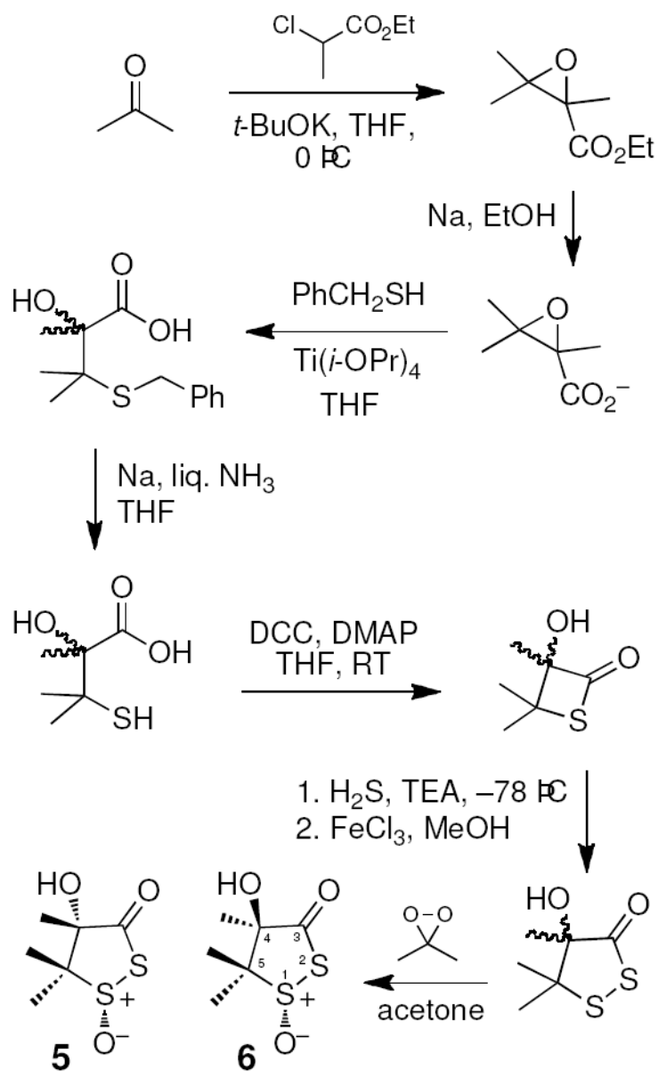
Scheme 2. Synthesis of 1,2-dithiolan-3-one 1-oxides related to leinamycin.
