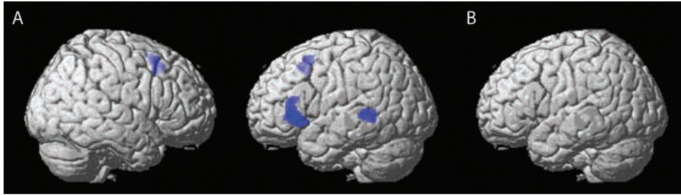
Figure 2. Whole-brain results (see also Table 1). (A) The adaptation effects for syntax repetition. In left MTG, left IFG, and supplementary motor area, there was a repetition suppression effect for repeated compared with novel syntactic structures. (B) Interaction between syntax repetition and modality repetition. No regions showed an interaction between syntax repetition and modality repetition.
