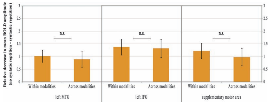
Figure 3. ROI analysis in the 3 clusters showing a main effect of syntactic repetition—left MTG, left IFG, and supplementary motor area—confirmed that there was no differential repetition suppression effect for syntactic structures within and across processing modalities.
