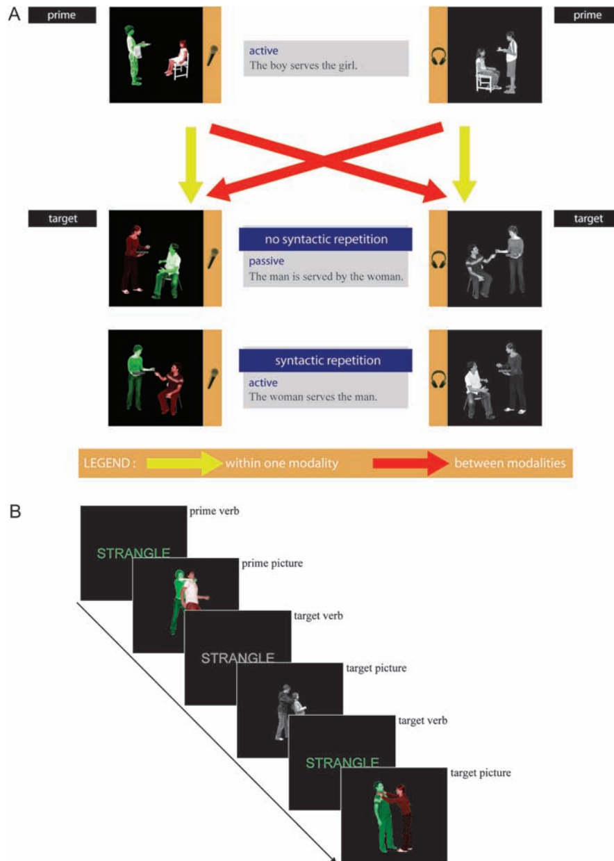
Figure 1. (A) Design and stimuli. Participants either described colored photographs or listened to descriptions of grayscale photographs, containing action, agent, and patient. To guide production, participants were instructed to name the green actor before the red actor. Between subsequent sentences, that is, prime and target, the syntactic structure and the processing modality could be repeated (for syntax: active–active or passive–passive, for modality: production–production or comprehension–comprehension) or novel (for syntax: active–passive or passive–active, for modality: production–comprehension or comprehension–production). (B) Procedure. We used a running priming paradigm where each target item also served as a prime sentence for the next target item. The verb always preceded the photographs. Green verbs indicated a “production photograph” would follow, gray verbs indicated a “comprehension photograph” would follow.
