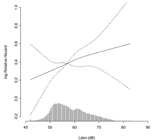
Figure 1. Association between road traffic noise and myocardial infarction. Association between exposure to road traffic noise ( L_{\text{den}} ) at the residence at the time of diagnosis and incident MI, adjusted for sex, smoking status, smoking duration, smoking intensity, intake of fruit, vegetables and alcohol, BMI, physical activity, calendar year, education, railway and airport noise, and air pollution. Solid line: incidence rate ratio, dashed lines: 95% confidence interval. The median (56.4 dB) is the reference. The columns at the x-axis show the distribution of exposure to road traffic noise. doi:10.1371/journal.pone.0039283.g001
