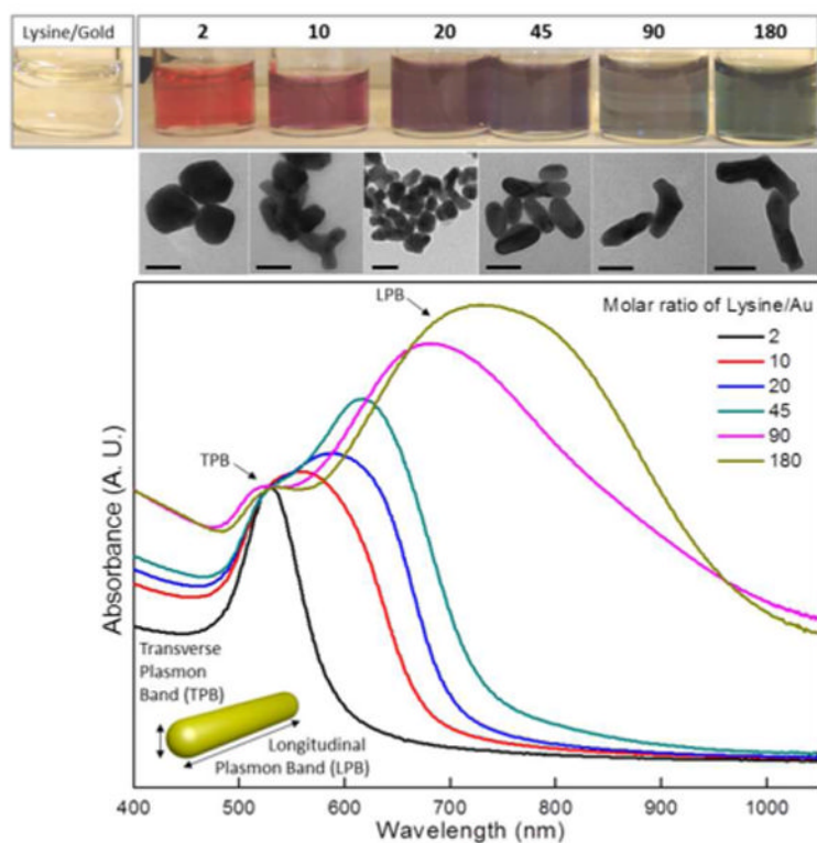
Fig. 1. Absorption spectra and TEM images of the gold nanorods (GNRs) grown with varying amounts of the lysine/gold precursor (Lys/Au) ratio. Various colors of the GNR solutions correspond to the absorption spectra of different Lys/Au ratios (top). Corresponding TEM images showing structural evolution (middle, also see Fig. S1). Scale bar is 30 nm.
