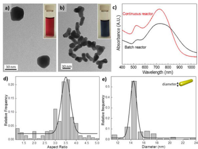
Fig. 2. TEM images and absorbance spectra of the Au nanostructures. (a) TEM image of Au nanostructures obtained at Lys/Au molar ratio of 2, in a batch reactor. (b) At molar ratio of 180, in a continuous flow reactor. Insets of (a) and (b) Optical images from gold colloids obtained at different Lys/Au ratios. (c) Comparison of absorbance spectra from GNRs obtained in a batch reactor and continuous flow reactor (oxidant flow rate of 40 \mu\text{L}/\text{min} and reductant flow rate of 10 \mu\text{L}/\text{min} ) with same Au/Lys molar ratio of 180. (d), (e) Statistical analysis of produced GNRs obtained in continuous flow: (d) aspect ratio and (e) diameter.
