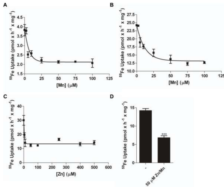
Fig. 5. Mn II and Zn II partially inhibit the uptake of ferrous iron by hBMVEC
