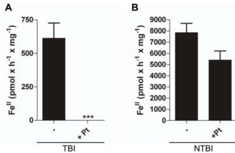
Fig. 3. Reduction of TBI and NTBI is dependent upon hBMVEC-surface ferrireductases Colorimetric ferrozine assays were used to quantify the formation of Fe II species in solution. Each sample was blank corrected with a minus hBMVEC control and normalized for protein concentration. Potassium tetrachloroplatinate II (100 \mu M) was used to inhibit reductase activity by hBMVEC. Substrates were either TBI (a) or NTBI (b). Values are mean \pm SD (a, n =12; b, n=3). ***P-value < 0.0001 as analyzed by the paired t-test.
