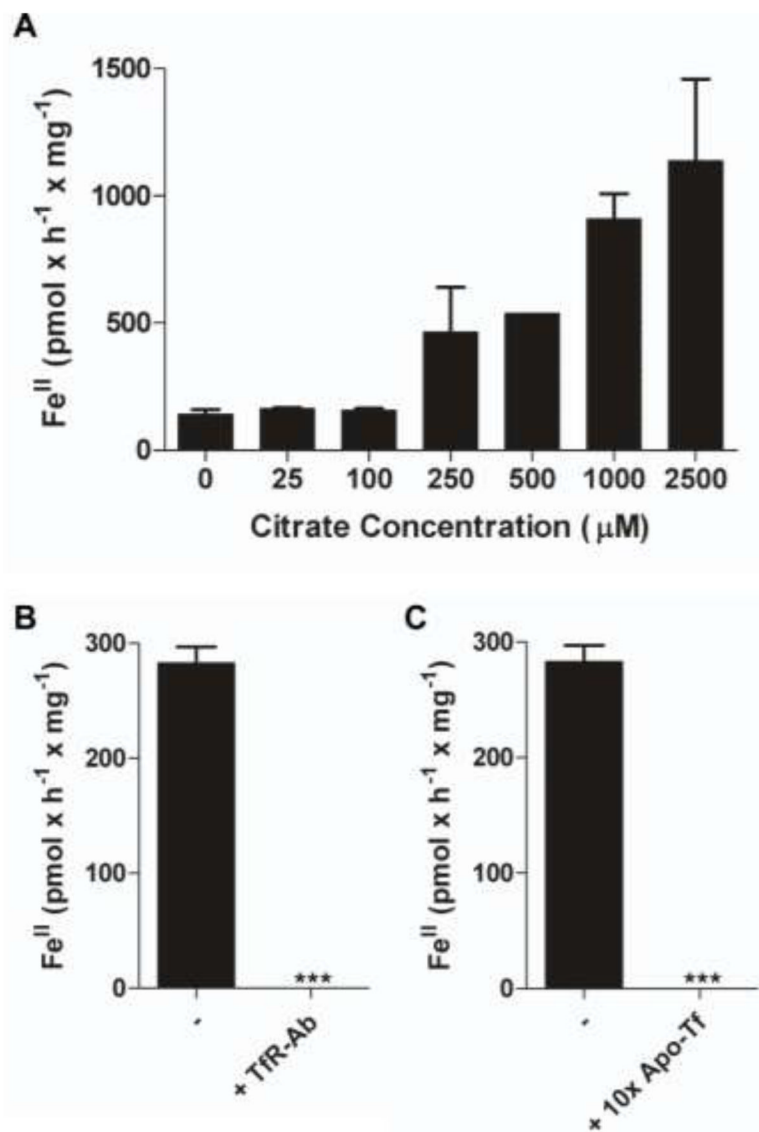
Fig. 2. Reduction of TBI is dependent upon citrate concentration and Tf-TfR interaction The hBMVEC- dependent formation of Fe II species were quantified using colorimetric ferrozine assays. Each sample was blank corrected with a minus hBMVEC control and normalized for protein concentration. Monolayers of hBMVEC were incubated with TBI, ferrozine, and either increasing concentrations of citrate (a), anti-TfR antibody (b), or 10-fold apo-Tf (250 μM) (c). (b and c) contained a constant citrate concentration. n = 3 for each result in each panel. Data are mean ± standard deviation (SD). ***P-value < 0.0001 as analyzed by the paired t-test.
