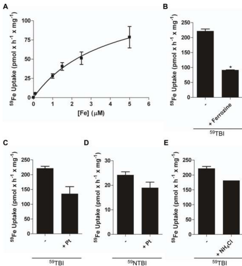
Fig. 4. Both TBI and NTBI are substrate for endosomal-independent hBMVEC iron uptake A \gamma counter was used to quantify the amount of 59 Fe uptake by hBMVEC monolayers. The kinetics of 59 Fe II -citrate plus Asc accumulation by hBMVEC are shown (a). Data are shown representing hBMVEC accumulation of 59 Fe from 59 Fe-Tf in the presence ferrozine (b) or Pt II (c). 59 NTBI uptake in the presence of Pt II was also monitored (d). Effect of hBMVEC-alkalinization via NH 4 Cl on 59 TBI accumulation was quantified and compared to control (e). n = 3 for each result in each panel. The Michaelis-Menten equation was used to calculate the curve (a). Data are mean \pm SD. *P-value < 0.01 as analyzed by the unpaired t-test.
