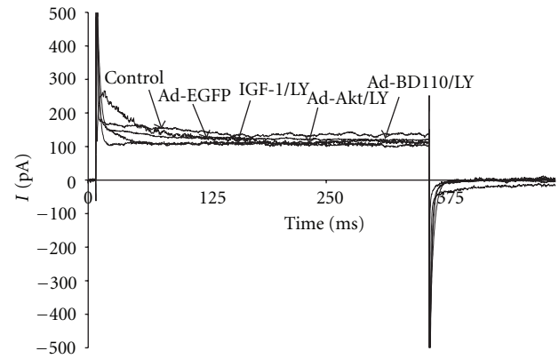
FIGURE 4: Recording representative of the time courses for the effects of IGF-1, Ad.Akt, and Ad.BD110 in combination with LY 294002 treatments on I_K of normal neonatal rat cardiomyocytes at the clamp voltage of +30 mV. Current expressed as pA.
