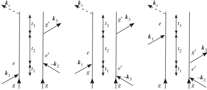
Figure 2. The three double-sided Feynman diagrams that represent the same process as the single-loop diagram used in figure 1.
