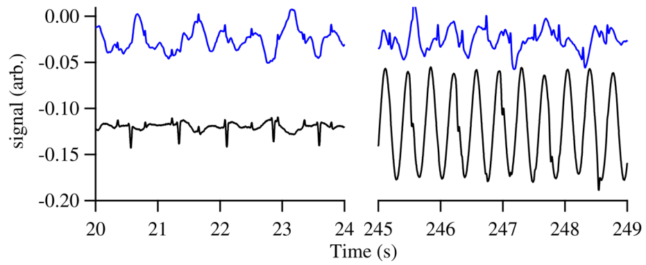
Fig. 4. (Color online) Two feedback scenarios. The lower trace is the current supplied to the large field coil to hold the signal constant at channel 4. The upper trace shows the field at another channel. (left) Data with a nearby ventilation fan off; the maternal signal is nearly the same size at the two channels, so it is largely absent from the upper channel. (right) With the fan on, the fMCG is still visible in the upper channel thanks to the feedback compensation.
