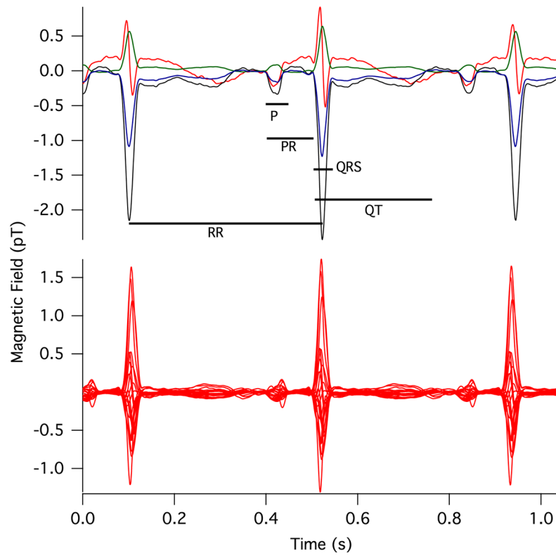
Fig. 3. (Color online) Comparison of the (top) prototype optical magnetometer and (bottom) commercial SQUID signals, with timings between features corresponding to Table 1.
