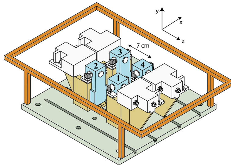
Fig. 1. (Color online) Biomagnetometer array. Four magnetometers are symmetrically located in the plane of a field coil. The output P_{I_x} of one magnetometer is fed back to actively null B_{I_y} . Each channel consists of a heated glass cell (numbered)
