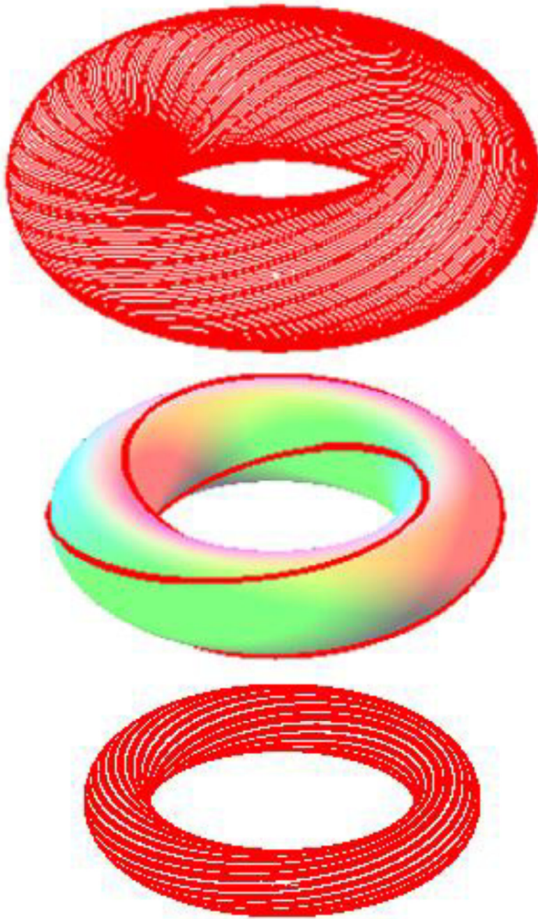
Fig. 4. Rational orbit with p = 2 and q = 3 (Middle, radius is I_B ) and two irrational orbits (Top and Bottom, radii are I_A and I_C respectively); I_A > I_B > I_C .
