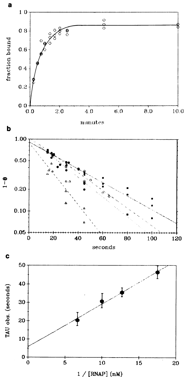
Figure 6. Association kinetics for RNA polymerase with rrpB P1. Kinetics were measured in the presence of ATP and CTP using the filter binding assay as described in Materials and Methods. Points from at least three separate
