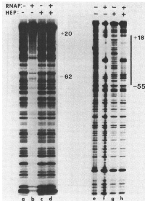
Figure 1. Competitor requirement for defined rRNA promoter - RNA polymerase complexes. Footprints were performed as described in Materials and Methods. The RNAP:DNA ratio was 5:1, the RNAP concentration was 10nM, and the heparin (HEP) concentration was 10 \mu g/ml. Lanes a-d: rrnB P1 promoter fragment (-152 to +50, labeled at the upstream site on the top strand). Lanes e-h: lacUV5 promoter fragment (-140 to +63, labeled at the upstream site on the top strand). Numbers refer to positions relative to the transcription start site and are shown only to orient the reader. No nucleotides were present in the reactions, so no specific footprint is seen in lane d. The line adjacent to lane h shows the approximate position of the footprints in lanes f and h.
