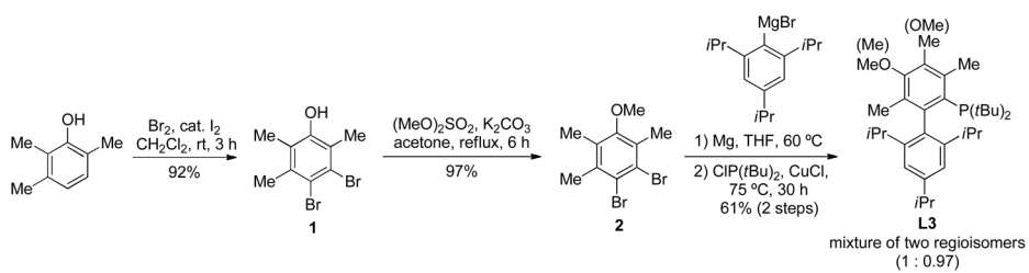
Scheme 1. Preparation of L3
