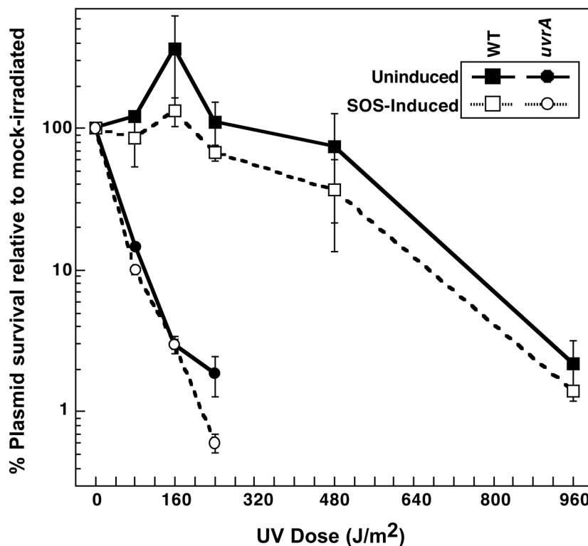
FIGURE 5. Constitutive recA expression does not enhance the survival of transforming UV-damaged plasmids
