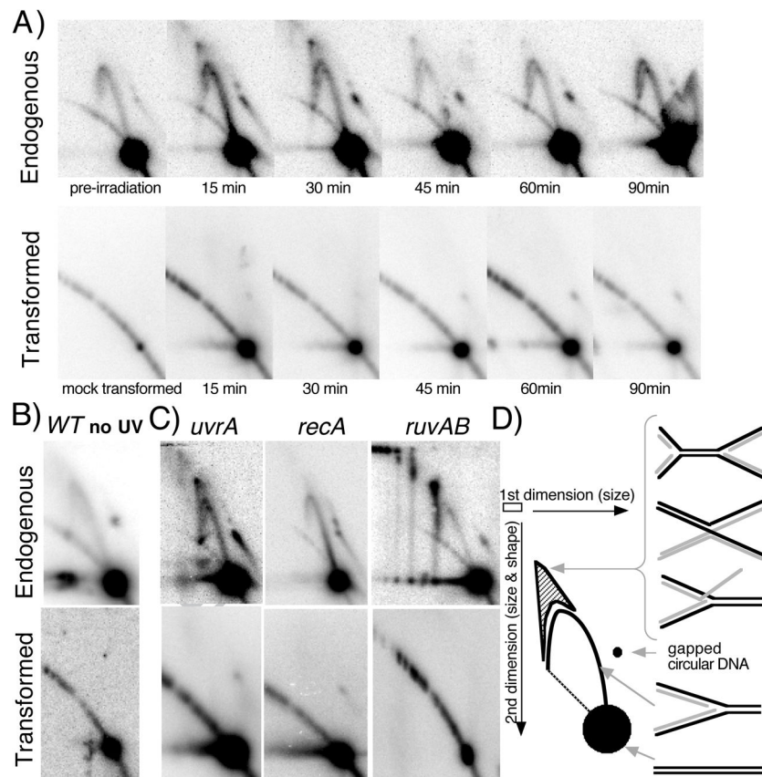
FIGURE 4. Replication- and RecA-dependent processing intermediates are not observed on newly introduced plasmids
