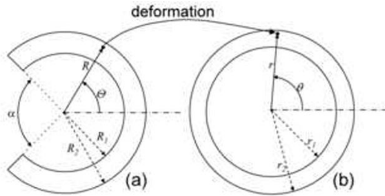
Figure 1. Deformation of arterial wall from open sector (zero-stress reference configuration) (a) to loaded state (b) under inner and outer constant hydrostatic pressures applied on the faces.
