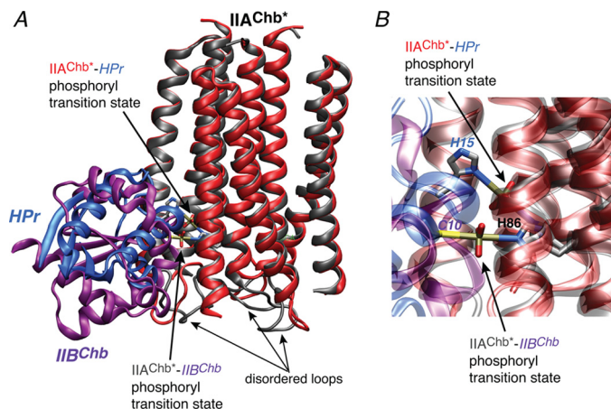
FIGURE 7. Comparison of the IIA Chb* -HPr and IIA Chb* -IIB Chb complexes. A , overall stereoview with IIA Chb* from the two complexes best-fitted to one another, and B , close up of the His-P-His and His-P-Cys phosphoryl transition states for the IIA Chb* -HPr and IIA Chb* -IIB Chb complexes, respectively. The backbone is displayed as a ribbon diagram and the His-P-His and His-P-Cys transition states as stick diagrams with the atoms color coded according to type (carbon, gray ; nitrogen, blue ; oxygen, red ; phosphorus, gold ; sulfur, yellow ). For the IIA Chb* -HPr complex, IIA Chb* and HPr are shown in red and blue , respectively; for the IIA Chb* -IIB Chb complex, IIA Chb* and IIB Chb are shown in gray and purple , respectively. The coordinates of the IIA Chb* -IIB Chb complex are taken from Ref. 43 (PDB code 2WWV). The small differences in the IIA Chb* coordinates from the two structures is within coordinate error. Also note that the region that displays the largest apparent differences is the loop from residues 77 to 84 of IIA Chb* , which is disordered in solution.
