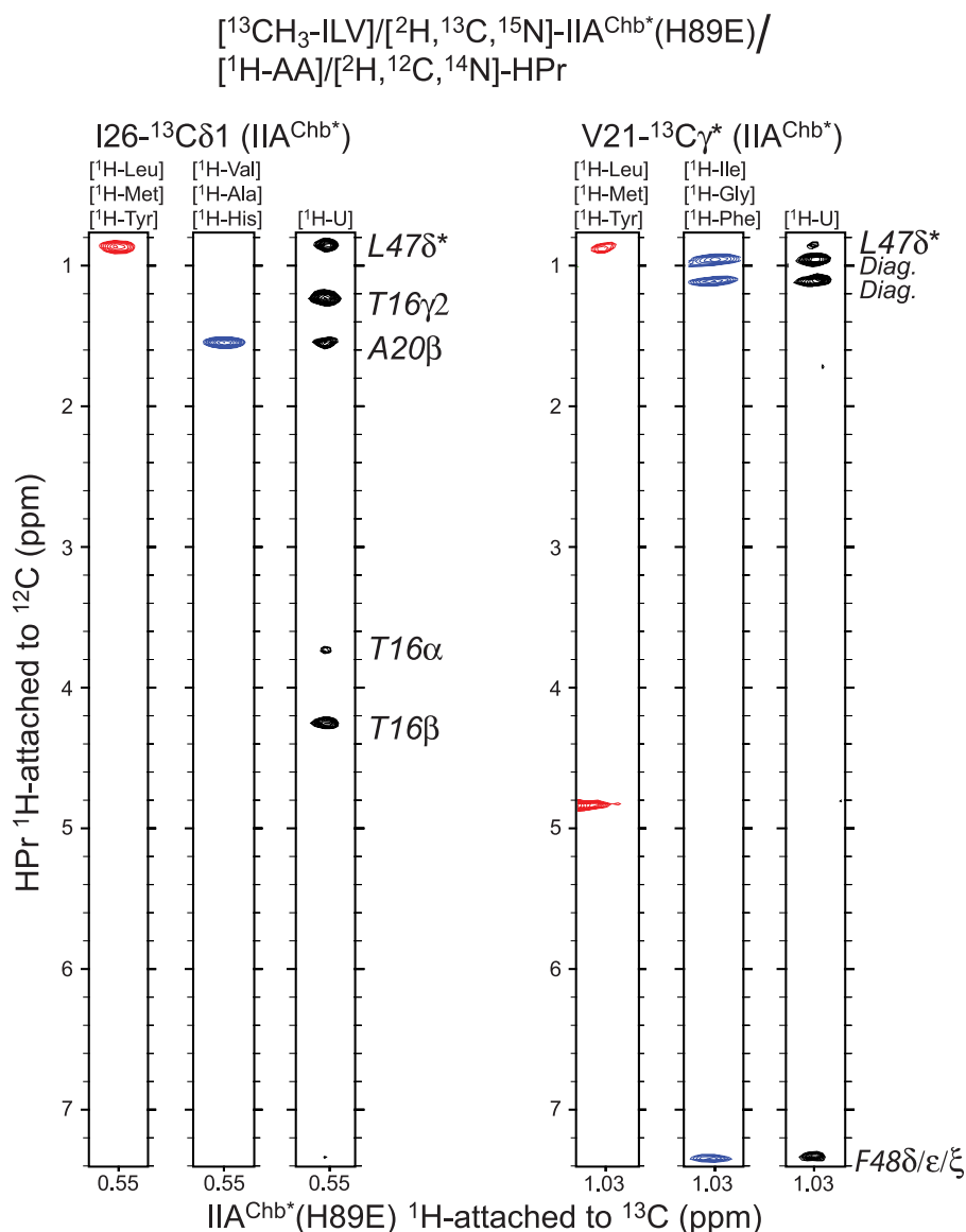
FIGURE 2. Intermolecular NOEs in the IIA Chb* (H89E)-HPr complex. NOEs in a three-dimensional 12 C-filtered/ 13 C-separated NOE experiment recorded in D 2 O are specifically observed from protons attached to 12 C (in the F 1 dimension) to methyl protons attached to 13 C (in the F 3 dimension). Strips are shown for NOEs involving the 13 Cδ1 methyl group of Ile-72 (at 12.48 ppm) and one of the 13 Cγ methyl groups of Val-21 (at 23.63 ppm) of IIA Chb* (H89E). The amino acid (AA) specific labeling schemes used for [ 1 H-AA]/[ 2 H, 12 C, 14 N]-HPr are shown above each strip.
