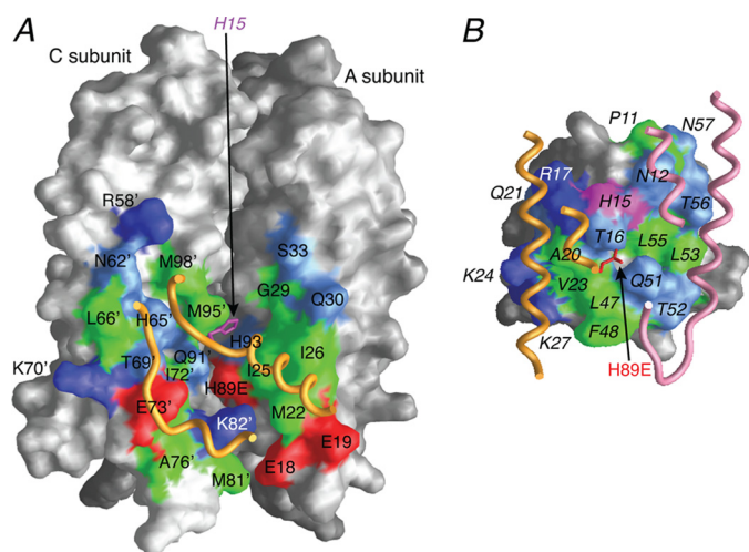
FIGURE 4. Interaction surfaces for the IIA Chb* (H89E)-HPr complex. A , interaction surface (formed by the A and C subunits) on IIA Chb* (H89E) for HPr. B , interaction surface on HPr for IIA Chb* (H89E). The surfaces are color coded as follows: hydrophobic residues, green; uncharged residues bearing a polar functional group, cyan; negatively charged residues, red; positively charged residues, blue. Relevant portions of the backbone and the active site residue of the interacting partner are displayed as tubes and bonds, respectively. Residues of HPr are labeled in italics . Residues from the C subunit of IIB Chb* (H89E) are indicated by an apostrophe after the residue number; in addition, the surfaces of the A and C subunits of IIA Chb* that do not constitute the interaction surface are colored in dark gray and light gray, respectively.
