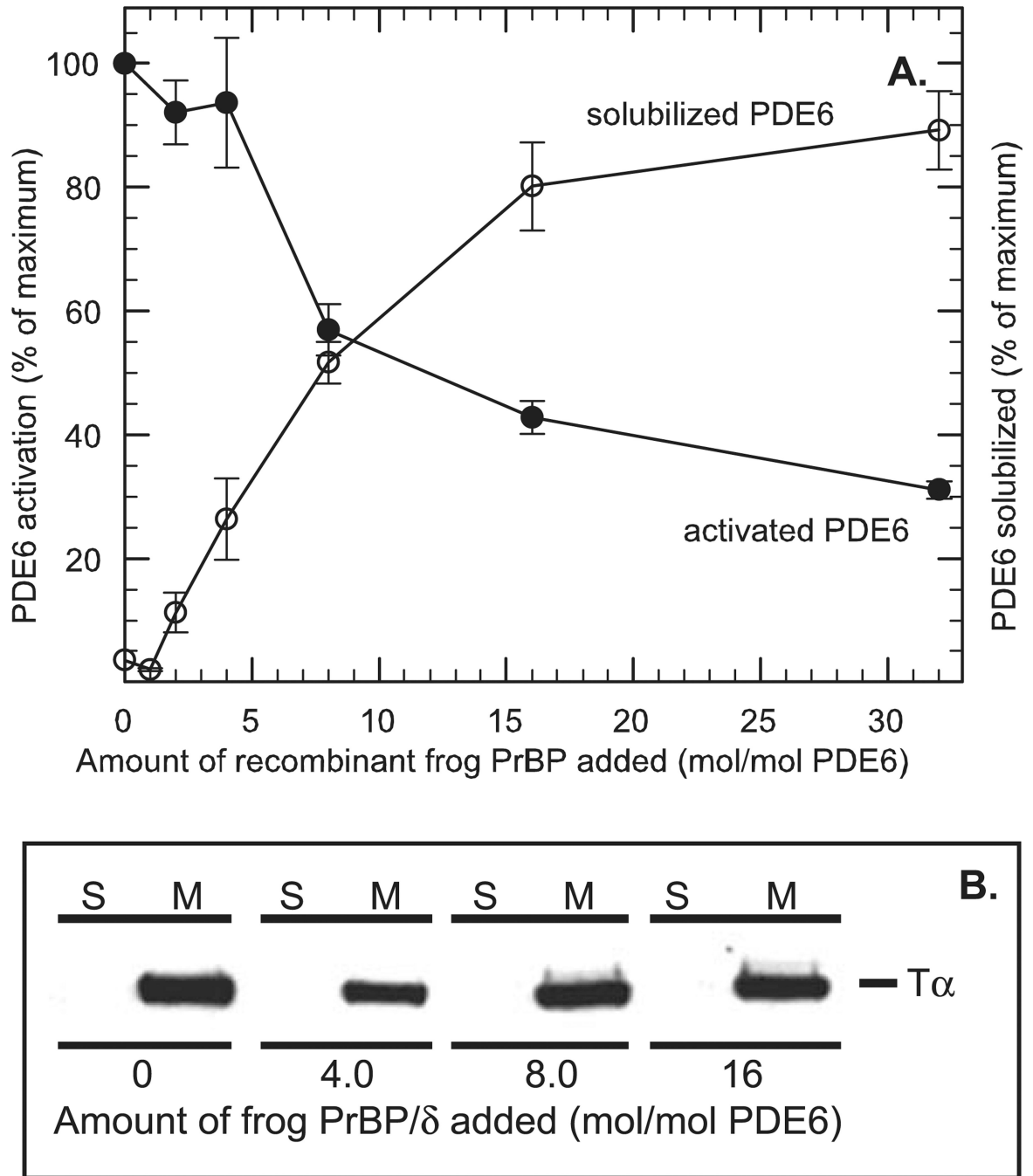
Fig. 4. PrBP/δ blocks transducin activation of PDE6 in vitro without releasing Tα*-GTPγS from ROS membranes
