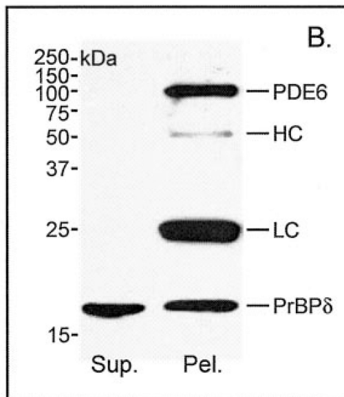
Fig. 3. Recombinant frog PrBP/δ solubilizes PDE6 from ROS membranes and forms a stable complex in vitro
