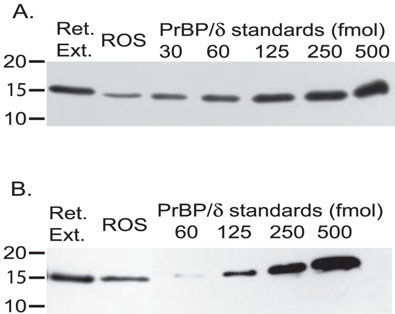
Fig. 6. Quantitating PrBP/ \delta content in retinal extracts and in ROS
