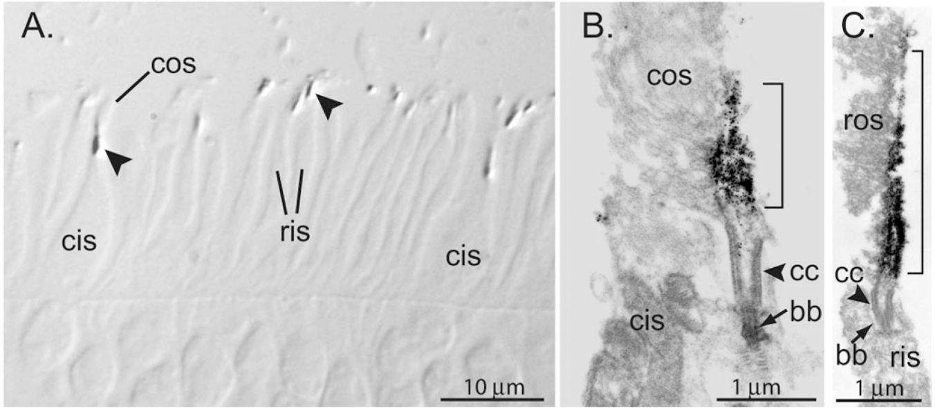
Fig. 9. Immunoelectron microscopy localizes PrBP/δ to the ciliary axonemes of bovine rods and cones
