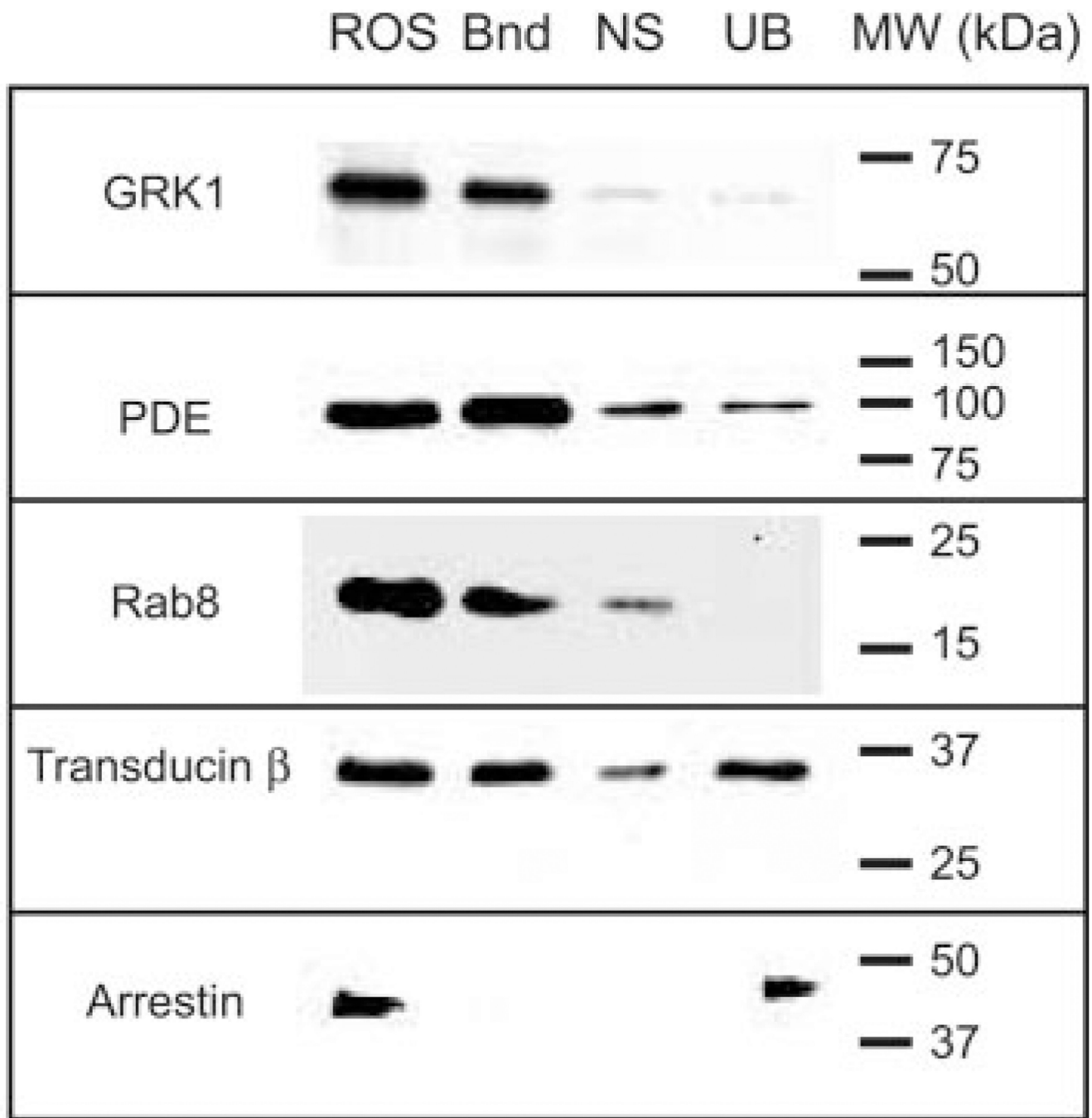
Fig. 5. PrBP/δ binds to several prenylated photoreceptor proteins in bovine ROS homogenates Detergent-solubilized bovine ROS (3.5 pmol of PDE6) were incubated with PrBP/δ-Sepharose (2 mg of PrBP/δ per milliliter of resin), and proteins bound to the resin ( Bnd ) were separated from unbound proteins ( UB ) by centrifugation. As a control for nonspecific binding to the resin ( NS ), identical samples were incubated with a large excess of PrBP/δ. Equivalent amounts of the starting sample ( ROS ) were also loaded. After SDS-PAGE and transfer to polyvinylidene difluoride, blots were probed with primary antibodies to GRK1, PDE6, Rab8, transducin \beta -subunit, and arrestin.
