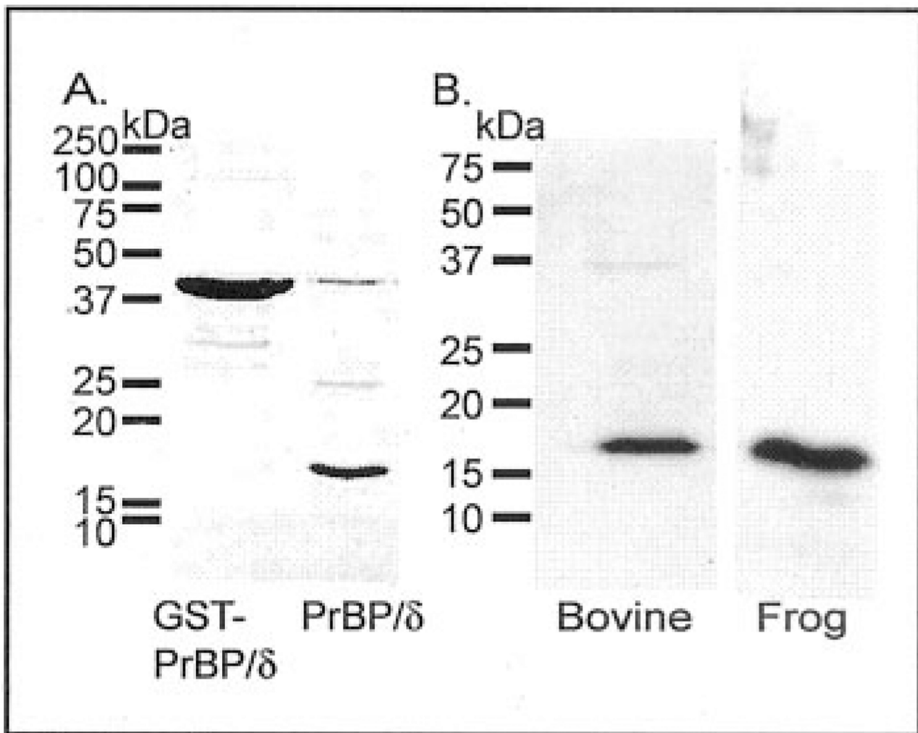
Fig. 2. Recombinant expression of frog PrBP/δ and antibody specificity of the PrBP/δ antibody (FL)
