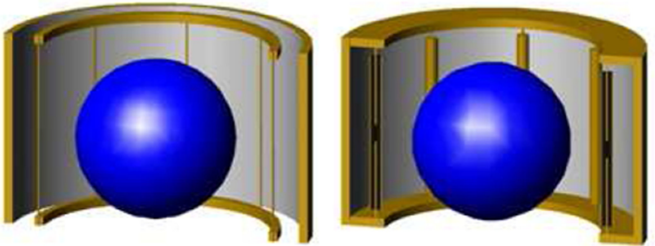
Figure 1. Geometry of the birdcage coil (left) and TEM-type resonator (right) loaded with the spherical sample for the first group of calculations.
