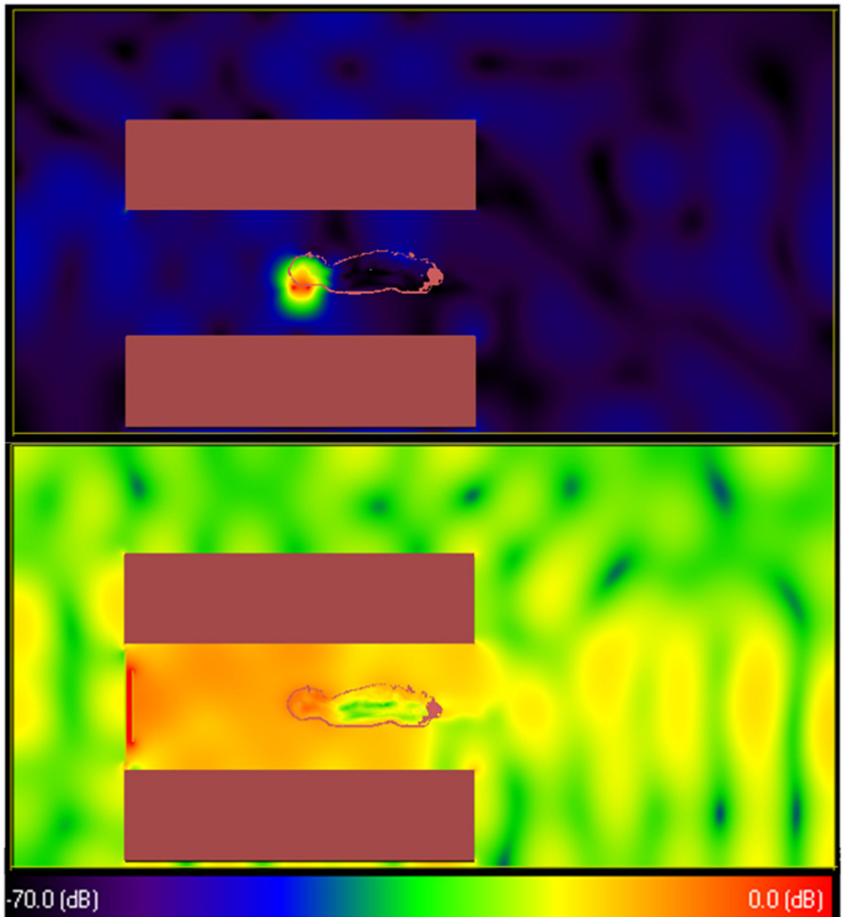
Figure 2. Geometry and B_1 field distribution on mid-sagittal plane for the most complete case in calculations involving a surface coil (second group of calculations) and patch antenna (third group of calculations) at 300 MHz. Fields are scaled to have a \|B_1\| of 2\mu\text{T} at the center of the brain, and the maximum value of the logarithmic color scale (0dB) is 10\mu\text{T} .
