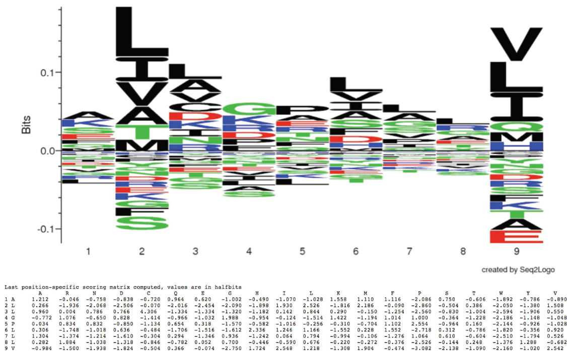
Figure 2. Output from Seq2Logo. The upper panel shows the sequence logo calculated from a set of 13 artificial peptide sequences using the specification defined in Figure 1 (sequence weighting using clustering, pseudo count with a weight of 200 and logotype as Kullback-Leibler). Enriched amino acids are shown on the positive y-axis and depleted amino acids on the negative y-axis. The lower panel gives the position-specific (log-odds) scoring matrix (PSSM) calculated by Seq2Logo. Each line corresponds to a position and gives the consensus amino acid and the log-odds scores for the 20 amino acids.
