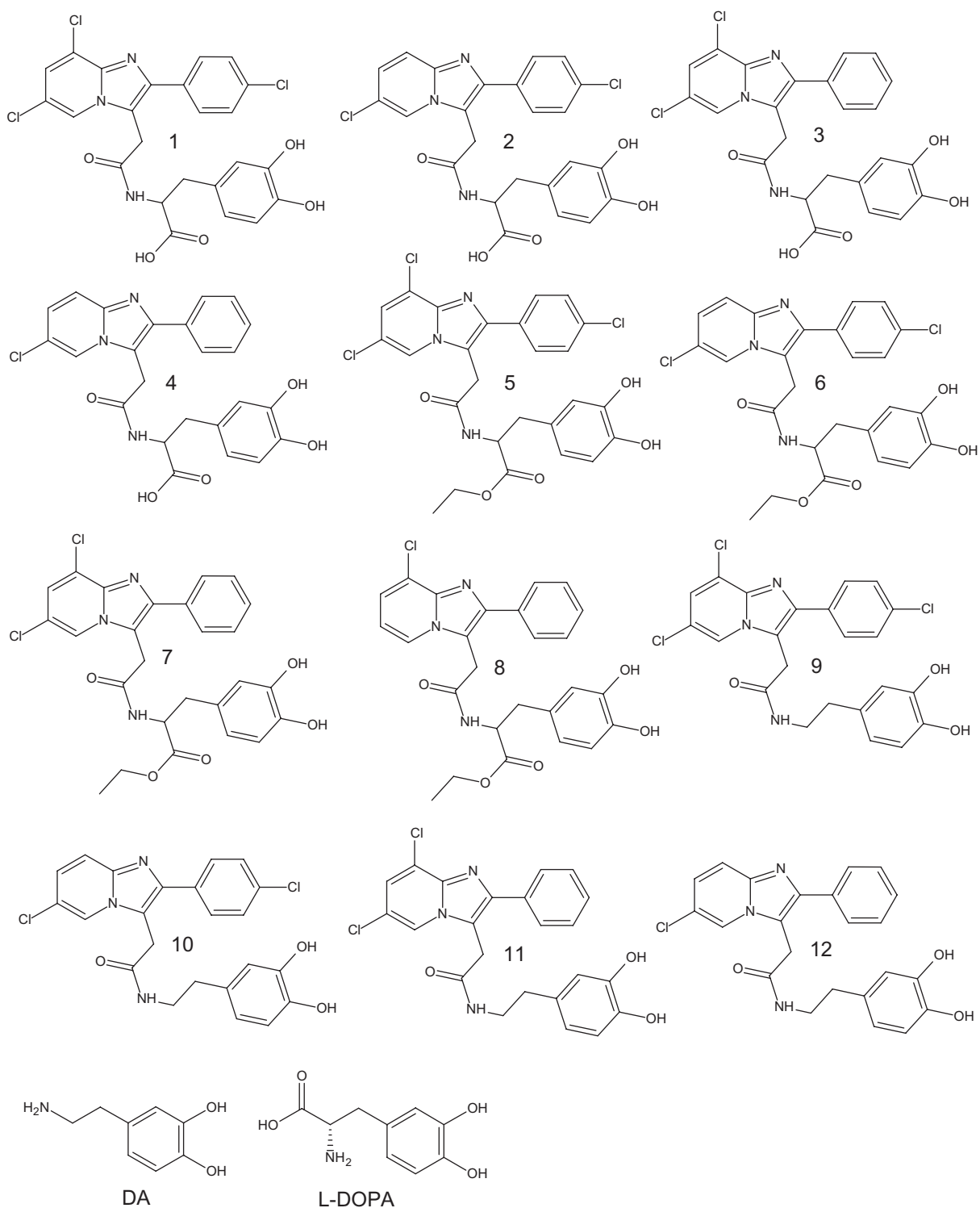
Figure 1 Chemical structure of DA, L-DOPA, and Dopimid compounds. Abbreviations: DA, dopamine; L-DOPA, levodopa.
