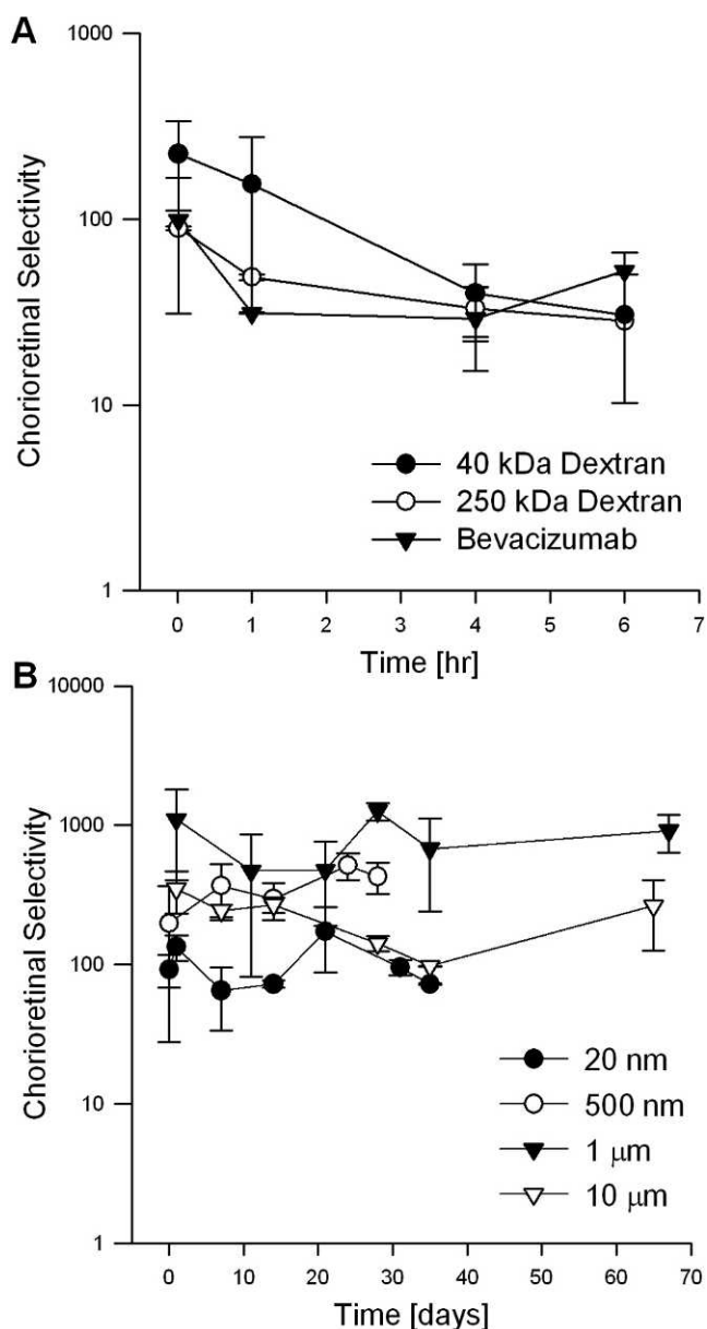
FIGURE 7. A comparison of the targeting of macromolecules (A) and particles (B) to the choroid and retina resulting from SCS administration in the rabbit eye in vivo. The chorioretinal selectivity is defined as the ratio of fluorescence intensity observed at the choroid and retina over what is observed at the lens. SCS administration of these materials results in a selectivity above 10 for the time periods tested. Data points represent average ( \pm SD), n = 2-3 .
