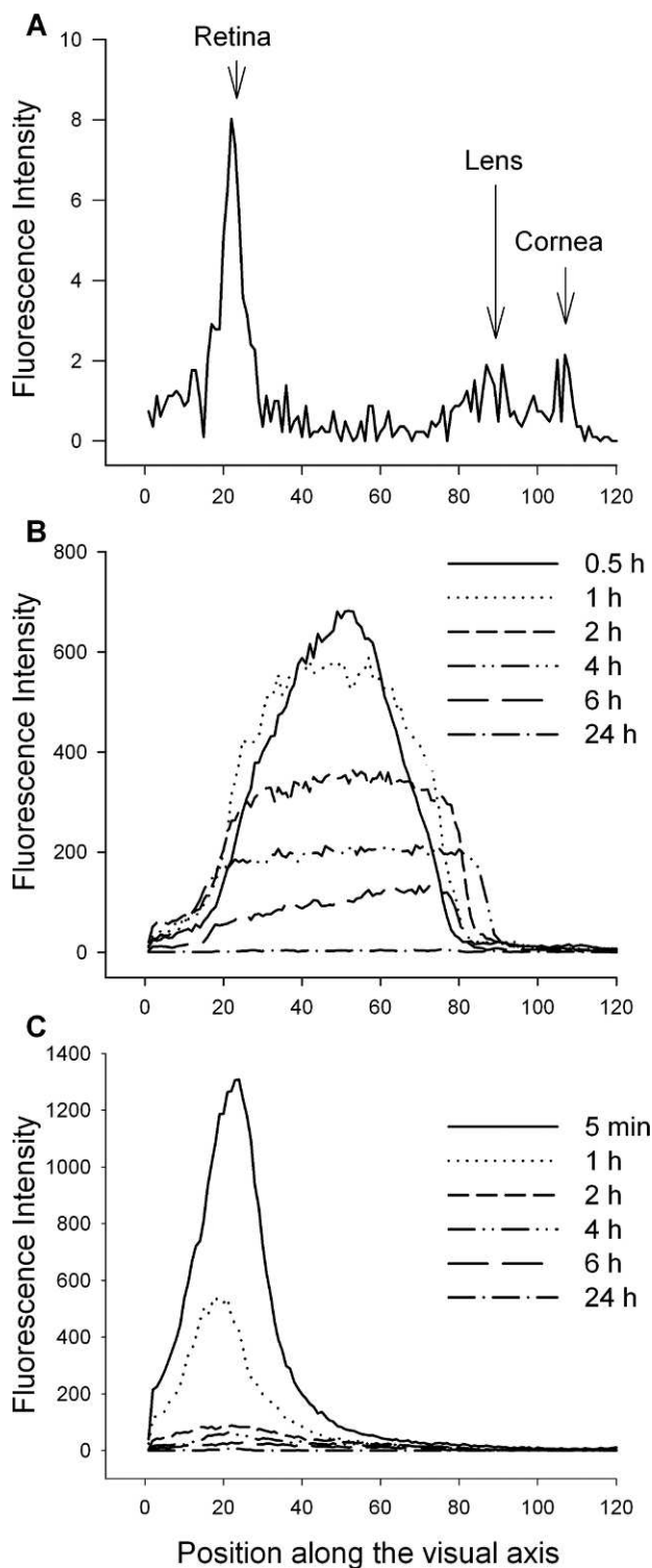
FIGURE 3. Fluorescence scans along the visual axis of the rabbit eye in vivo. A baseline scan of an untreated eye (A) delineates the retina, lens, and cornea of the eye owing to their natural background fluorescence. Intravitreal injection of NaF (B) caused an increase in the fluorescence intensity primarily within the vitreous that distributes uniformly throughout the vitreous and decays over time. Injection of NaF into the SCS (C) caused a sharp peak near the retina with a dramatically different profile than intravitreal injection. The NaF levels declined over a few hours and returned to baseline levels within 24 hours after both injections. Representative data are shown from three eyes at each condition.
