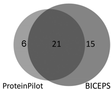
FIG. 6. L. sigmodontis protein identification using a B. malayi database. The Venn diagram shows the overlap of identified proteins at a 1% protein FDR level between ProteinPilot in its error-tolerant mode and BICEPS. While showing a strong overlap with ProteinPilot (27 proteins), BICEPS identifies 33% more proteins (36 proteins).
