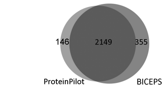
FIG. 5. Chinese hamster protein identification using a rat database. The Venn diagram shows the overlap of identified proteins at a 1% protein FDR level between ProteinPilot and BICEPS for the Chinese hamster ovary sample searched against the rat database. ProteinPilot (2,295 proteins) and BICEPS (2,504) show a large overlap with BICEPS identifying more proteins.
