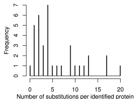
FIG. 7. Number of substitutions per protein identified by BICEPS on the L. sigmodontis data set. We observed an average of 6.1 substitutions per protein, which was identified in an error-tolerant search against the B. malayi database with an overall range of 0–20 substitutions.
