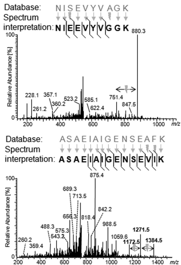
FIG. 4. Example of MS 2 spectra for peptides with two substitutions identified by BICEPS. In the case of the upper spectrum , we see strong evidence supporting the first substitutions (Ser to Glu). Both fragment ion series support the identification as indicated by the upper and lower diagonal lines in the sequence representation. In contrast, there is only limited direct evidence supporting the Ala to Gly substitution with general few clear signals in the corresponding spectral region. However, the precursor mass and the observed fragment ions provide very strong support for the indicated substitution. In the case of the lower spectrum , we see clear evidence in the spectrum for both substitutions occurring at the end of the sequence with clear spacings in the y ion series as indicated by the bolts . Additional examples are given in the supplemental material .
