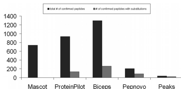
Fig. 3. Total number of confirmed peptides at a 5% FDR cutoff on the chicken database and number of confirmed peptides containing at least a single substitution. All of the confirmations are based on independent searches on the human database. BICEPS shows the highest number of confirmed peptides, as well as the highest number of confirmed peptides containing substitutions. Mascot searches do not result in any peptides with confirmed substitutions.
