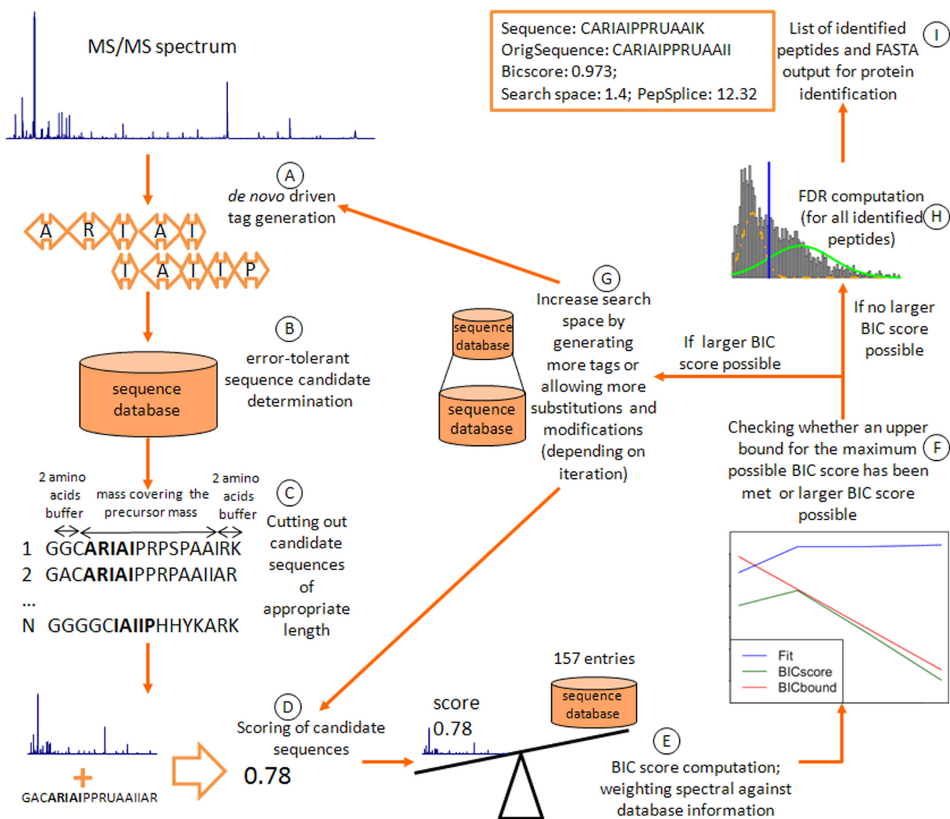
FIG. 1. Flow chart of the proposed workflow from tag generation through scoring and complexity estimation to confidence level estimation. After de novo tag generation (A), error-tolerant sequence candidates are determined (B), and peptide sequences of appropriate length are extracted (C). The resulting matches to the spectrum are scored (D) and weighted against the size of the search space using the BIC score (E). An early termination criterion allows abortion of the search without requiring the full search space (F). However, when better suited candidates may still be available, a deeper search with more tags or increased error tolerance is started (G). We apply a mixture model strategy to determine a confidence level estimate (H) and aggregate the results to identify proteins (I).
