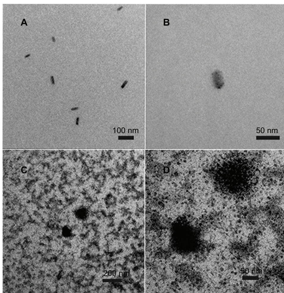
Figure 1 Transmission electron microscopy image of the physical state of C_{60}(OH)_x(ONa)_y . (A) Image of 1 \mu M fullereneol in water. (B) Amplified image of 1 \mu M fullereneol in water. (C) Image of 200 \mu M fullereneol in water. (D) Amplified image of 200 \mu M fullereneol in water.
