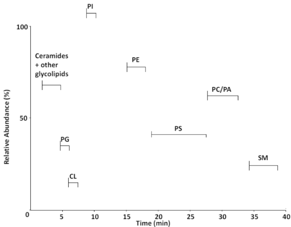
Figure 1. First-dimension (1D) separation of rat brain phospholipids by normal-phase HPLC-MS/MS
