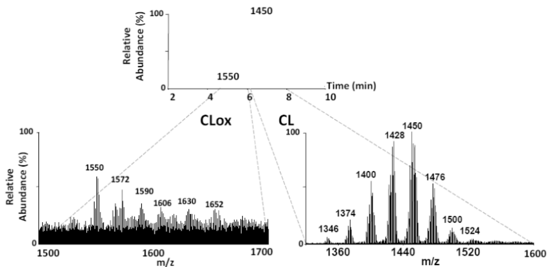
Figure 8. Assessment of oxidized CL species in normal rat brain tissue
