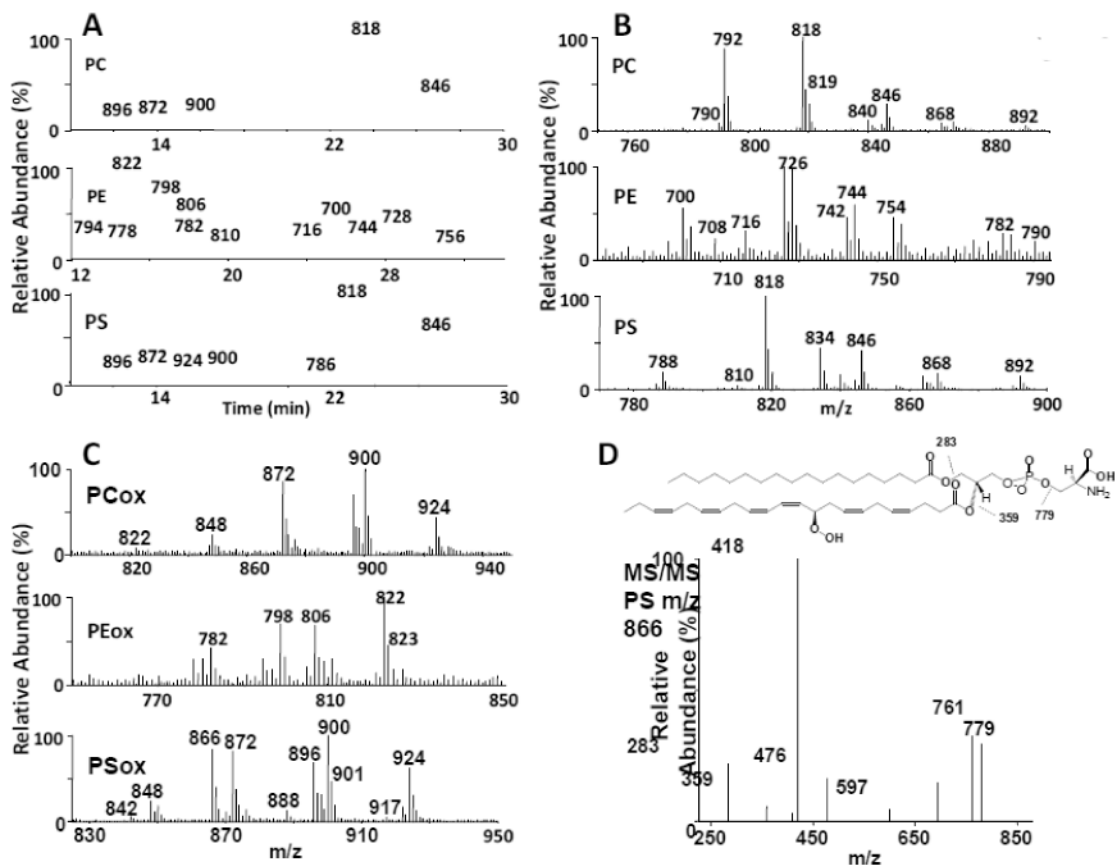
Figure 3. Second dimension (2D) analysis of brain PC, PE and PS oxidized in the presence of lipoxygenase
