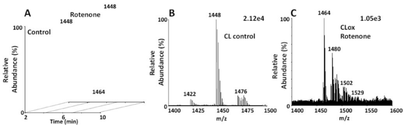
Figure 5. Treatment of human lymphocytes with rotenone induces monohydroxy and monoperoxy modifications of mitochondrial CL
