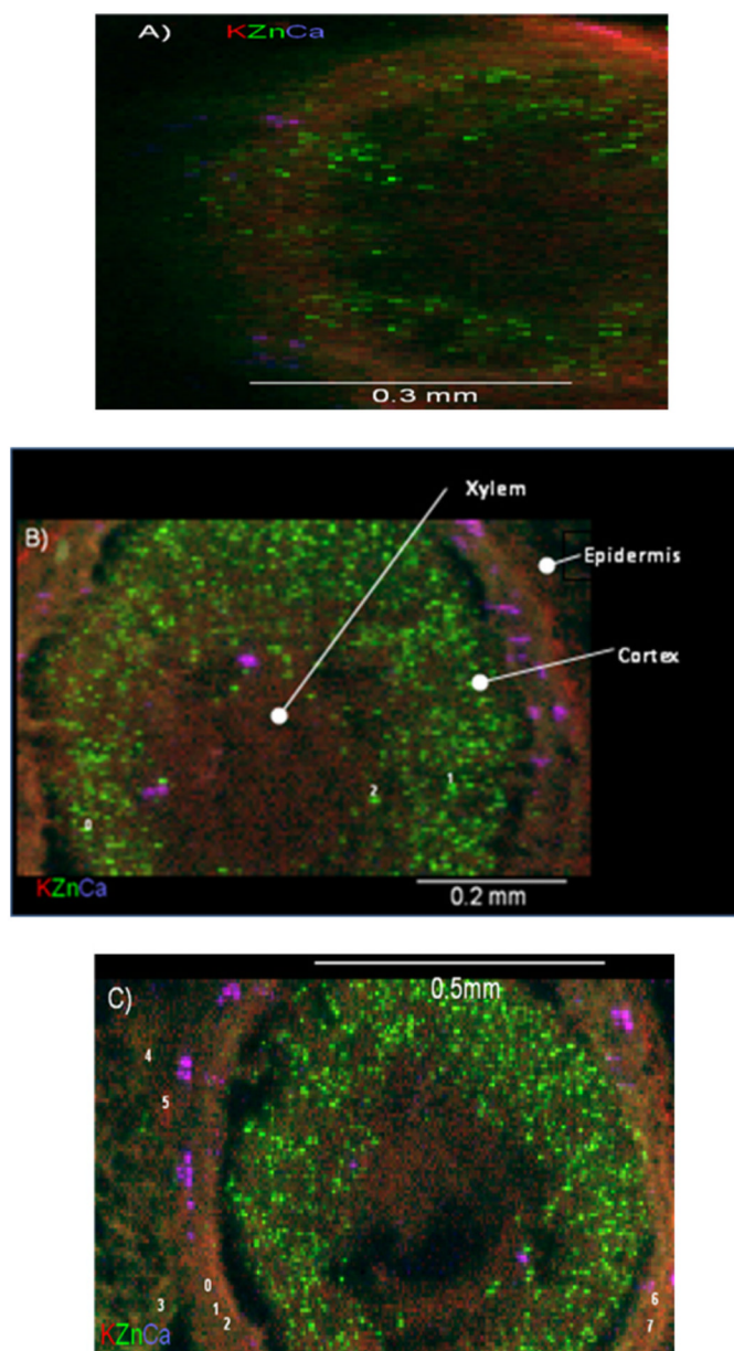
Fig. 4. Tricolour micro-XRF images of the cross sections of (A) mesquite root control (sample of 100 \mu\text{m} of thickness); (B) and (C) two different mesquite roots samples treated with 1000 \text{mg L}^{-1} (sample of 30 \mu\text{m} of thickness). Red colour stands for potassium, green for zinc, and purple for calcium. In (B) and (C), bright spots are labelled with numbers from 0 to 2 and diffused spots with numbers 0 to 7. (For interpretation of the references to colour in this figure legend, the reader is referred to the web version of the article.)
