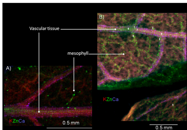
Fig. 5. Tricolour micro-XRF images of (A) mesquite leaves control and (B) mesquite leaves treated with 1000 mg L -1 . Red colour stands for potassium, green for zinc, and purple for calcium. In (B), bright spots are labelled with numbers from 0 to 5 and diffused spots with numbers 6 to 8. (For interpretation of the references to colour in this figure legend, the reader is referred to the web version of the article.)
