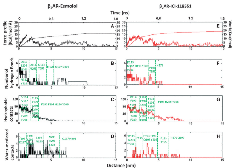
Figure 8. Esmolol and ICI-118551 unbinding from the \beta_2 adrenergic receptor on the example of one representative trajectory shown in the form of the rupture force, work, hydrogen bonds, hydrophobic and water-mediated contacts projected onto unbinding time and antagonist separation time from the initial position.
