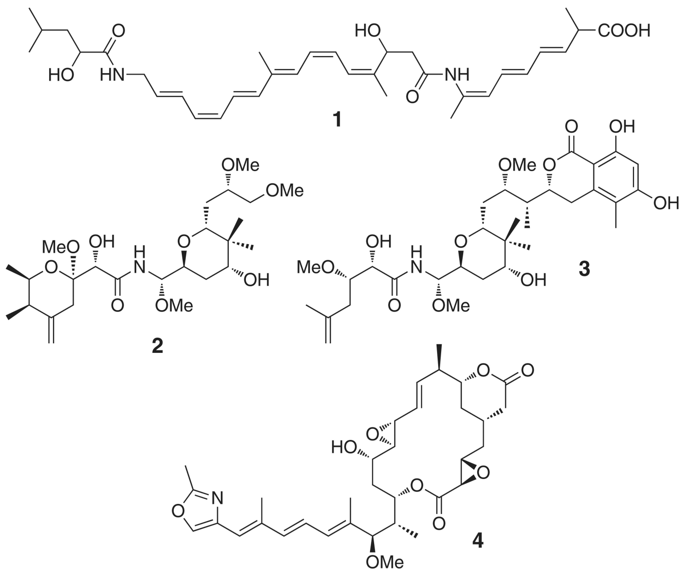
Figure 1. Selected Products of Trans -AT PKS Pathways Compounds are bacillaene (1), pederin (2), psymberin (3), and rhizoxin (4).
