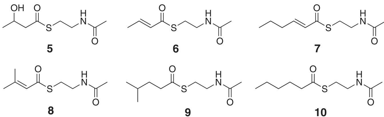
Figure 2. SNAC Derivatives Tested in the Hydrolysis Assays
