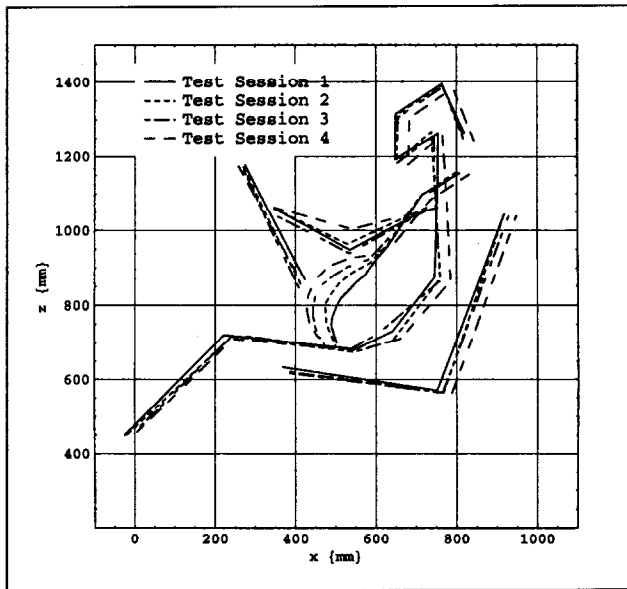
Figure 4. Average posture of Group-2 subjects for each test session at mid-seat-height conditions.
