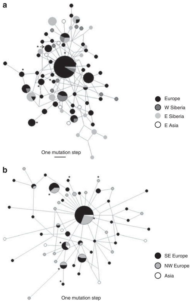
Figure 2 Unrooted median-joining networks based on 1162 bp sequences of the mitochondrial control region for (a) breeding ( n=162 ) and (b) wintering ( n=138 ) tufted ducks. Samples from the breeding season were grouped as Europe, Western Siberia (west of river Ob), Eastern Siberia and Eastern Asia. Wintering ducks were partitioned into hypothetical subpopulations in south-eastern and north-western Europe and in Asia (Iran, China and Japan). The size of the circles is proportional to the number of individuals with a particular haplotype. Asterisks mark the haplotypes observed in H5N1-positive tufted ducks sampled on European wintering grounds (see text). Note that the corresponding haplotypes are also indicated in (a) to illustrate their spatial distribution on the breeding grounds.
