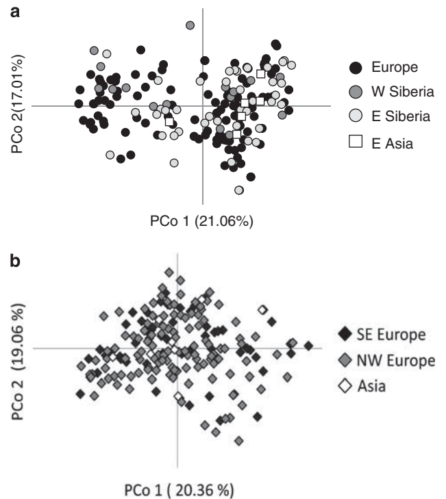
Figure 3 Plots of the first two coordinates from a principal coordinates analysis based on Euclidian distances between multi-locus microsatellite genotypes for (a) breeding individuals ( n=180 ) and (b) wintering individuals ( n=186 ) of tufted duck. Different symbols represent different geographic regions (see legend of Figure 2 for details).
