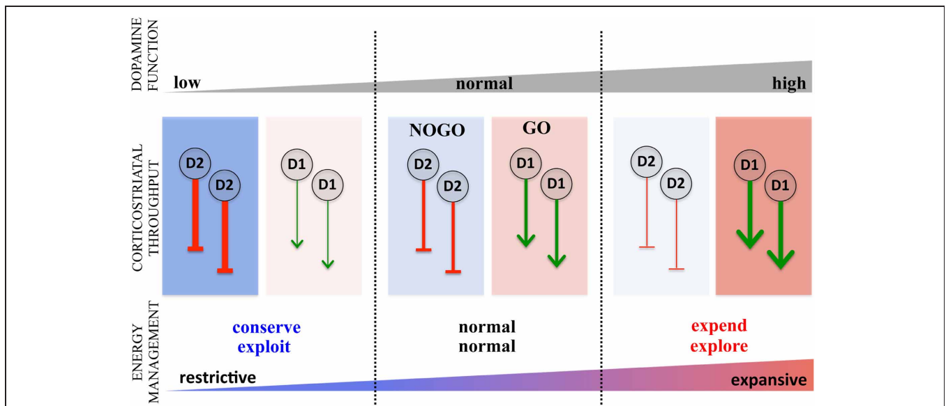
FIGURE 2 | Role of direct and indirect pathway modulation of corticostriatal throughput in regulating the energy expenditure.
