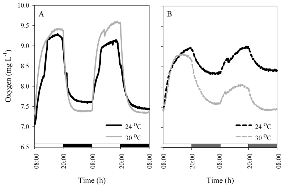
Figure 2 | Oxygen evolution of Stylophora pistillata corals during 2 LD cycles at 24 °C (continuous lines) followed by 2 cycles at 2 elevated temperatures 24 °C and 30 °C, (dashed lines). White bars: light period; black bars: dark period; grey bars: subjective darkness. For each time point, N = 4 . (A) corals under LD; (B) corals under LL.
