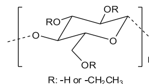
Fig. 16 Ethylcellulose structure
