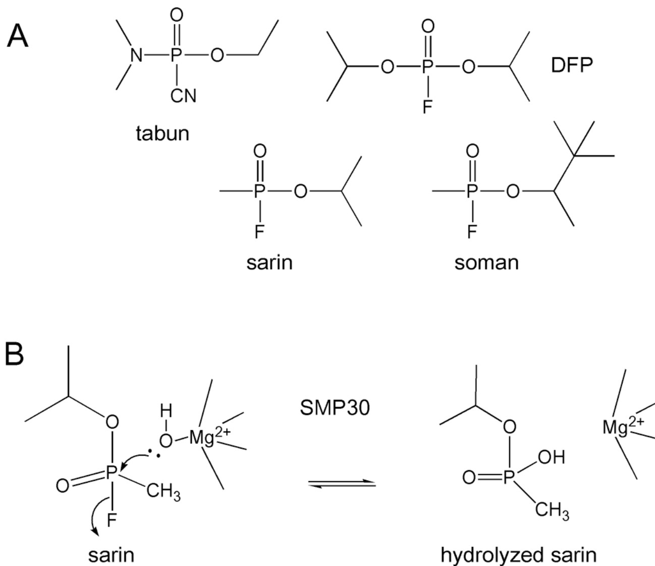
Figure 5. Organophosphates hydrolyzed by SMP30 (9). A) Structures of tabun, DFP, sarin, and soman. B) Hydrolysis of sarin by SMP30 and Mg^{2+} .
