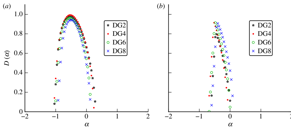
Figure 7. Wavelet choice: the multifractal singularity spectra computed from (a) measles incidence of infection data reported monthly in Ontario, Canada, from 1904 to 1989 and (b) the number of chicken pox cases reported weekly in Ontario from 1925 to 1958. Gaussian wavelets were tested against the data using an increasing number of vanishing moments. The order of the wavelet and thus the number of vanishing moments of the wavelet is given by the number of derivatives of the Gaussian. (Online version in colour.)
