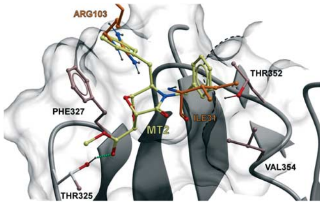
Figure 3 Binding sites of MT2 in TrkA molecule. In silico prediction of amino-acid residues involved. The predicted bound conformation of MT2 at the binding site of TrkA is shown. The surface of the pocket is reported explicitly with the structure of TrkA in gray ribbons as background. The amino acids of TrkA that establish direct interaction with MT2 are displayed in ball and stick representation. MT2 is displayed in ball and stick with carbon atoms colored dark yellow. As a term of comparison, Arg103 and Ile31 of NGF are reported in ball and stick with the carbon atoms colored orange. The H-bond between Thr325 of TrkA and MT2 is highlighted with green dots. The van der Waals volume of part of Thr352 and Val354 side chains is highlighted with a black dotted line
