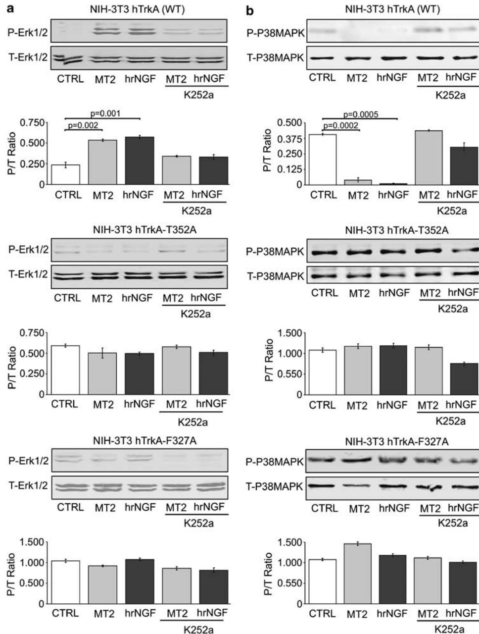
Figure 6 Biochemical pathways induced by MT2 in WT TrkA-NIH-3T3 or mutants. NIH-3T3 cells, stably transfected with full-length WT human TrkA, T352A, or F327A TrkA mutants, were cultured in serum-free medium and incubated with 10 \mu\text{M} MT2 or 4 \text{ nM} hrNGF, in the presence or absence of K252a. Cell lysates were blotted with rabbit anti-P-ERK (a) and anti-P-p38 MAPK (b). Then, membranes were stripped and stained with antibodies to the respective total protein. The relative histograms represent the densitometric analysis. Data are expressed as ratio between phosphoprotein (P) and total protein (T) of three different experiments (mean \pm S.E.). Statistical analysis was performed by paired Student's t -test
