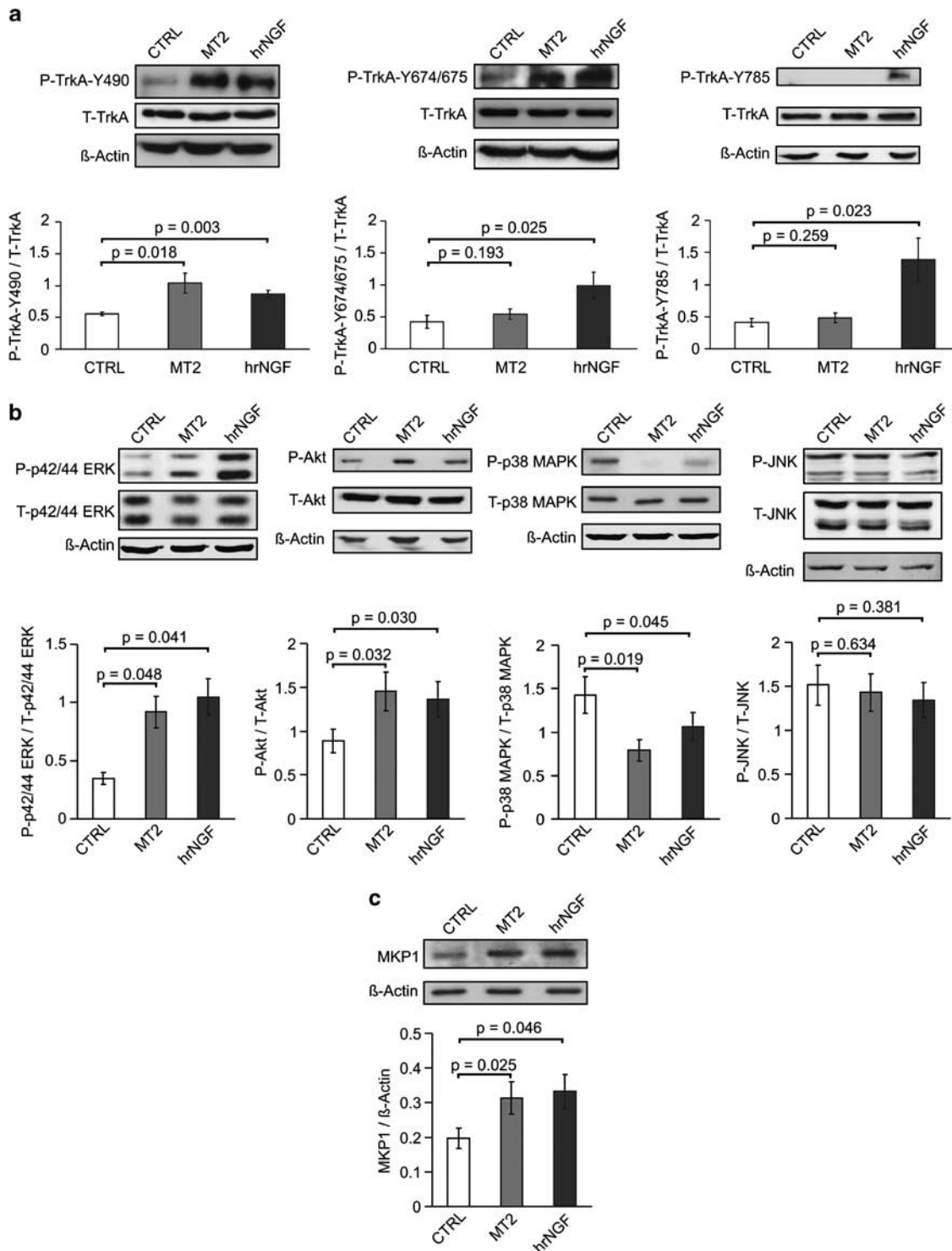
Figure 5 Biochemical pathways induced by MT2 in PC12 cells. (a) TrkA phosphorylation. Serum-starved PC12 cells were stimulated with 10 \mu M MT2, or 4 nM hrNGF as positive control, for 15 min. Cells lysates were blotted with antibodies to P-Y490, P-Y674/675, P-Y785 and with anti-actin as loading control. Membranes were stripped and stained with anti-total TrkA IgG. The relative histograms represent the data of densitometric analysis and are expressed as the ratio between phosphoprotein (P) and total protein (T) of five different experiments (mean \pm S.E.). Statistical analysis was performed by paired Student's t -test. (b) Kinases phosphorylation. Serum-starved PC12 cells were stimulated with 10 \mu M MT2, or 4 nM hrNGF, for 30 min. Cell lysates were blotted with rabbit anti-P-ERK, anti-P-Akt, anti-P-p38 MAPK, anti-P-JNK. Then, membranes were stripped and stained with antibodies to the respective total protein and with anti-actin antibodies as loading control. The relative histograms represent the data of densitometric analysis and are expressed as the ratio between phosphoprotein (P) and total protein (T) of five different experiments (mean \pm S.E.). Statistical analysis was performed by paired Student's t -test. (c) Phosphatase. Serum-starved PC12 cells were stimulated with 10 \mu M MT2, or 4 nM hrNGF as positive control, for 30 min. Cell lysates were blotted with rabbit anti-MKP1 IgG and anti-actin antibodies as loading control. The relative histogram represents the data of densitometric analysis and is expressed as the ratio between MKP1 expression and actin of five different experiments (mean \pm S.E.). Statistical analysis was performed by paired Student's t -test
