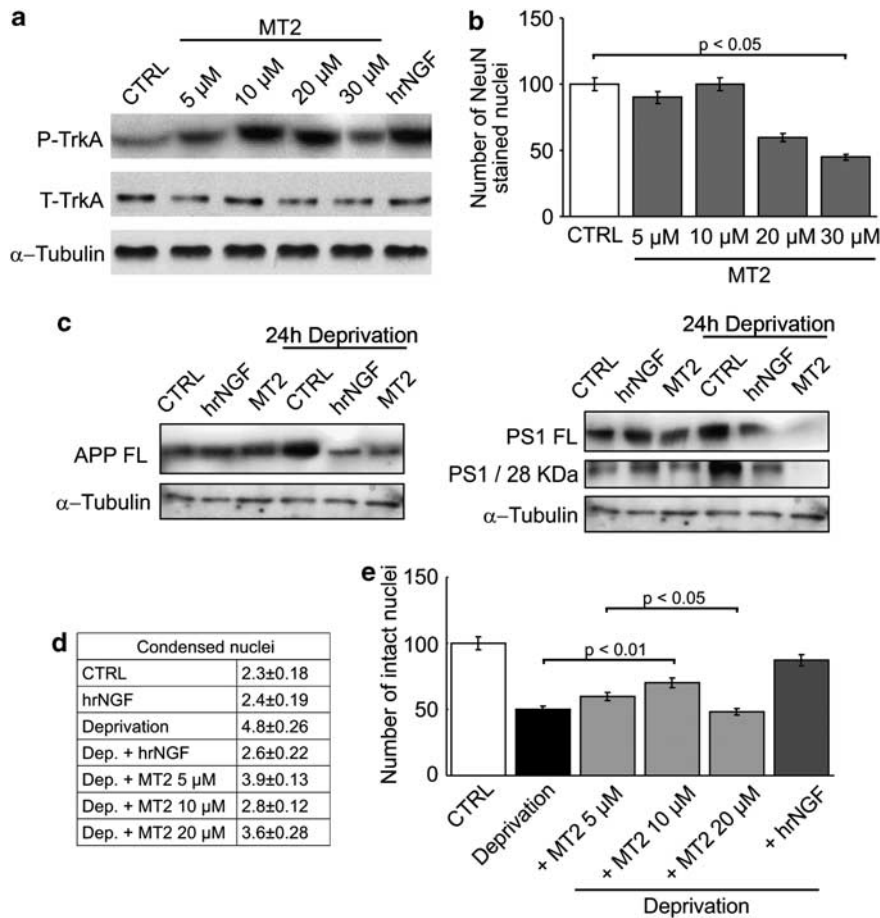
Figure 7 MT2 protects neurons from A \beta amyloid-mediated death in NGF-deficient neurons. (a and b) 3–4 days cultured hippocampal neurons were exposed to 2 nM NGF or to MT2 (5–30 \mu M) and the highest active concentration of MT2 evaluated as induction of TrkA phosphorylation by western blot analysis with anti-phosphorylated (P) and anti total (T) Trk-A antibodies or by counting the number of NeuN stained nuclei (b) . (c and d) hippocampal neurons were deprived of NGF by exposure to anti-NGF antibodies (30 \mu g/ml) for 24 h and incubated in the presence or absence of 10 \mu M MT2 or 2 nM hrNGF. Cells were lysed and western blot analysis performed with antibodies against APP full-length (c) and PS1 28 kDa N-terminal fragment (d) . (e and f) Hippocampal neurons were deprived of NGF by exposure to anti-NGF antibodies (30 \mu g/ml) for 24 h and then treated with concentrations of MT2 ranging from 5 to 30 \mu M or 2 nM hrNGF. The percentage of alive neurons was obtained by counting the number of intact nuclei (d) or alternatively by counting the number of condensed nuclei (e) . Ctrl, neurons not exposed to NGF or MT2; NGF, neurons exposed for 48 h to NGF; MT2, neurons exposed for 48 h to MT2 (10 \mu M); Dep, neurons deprived of NGF for 24 hours; Dep + NGF, neurons washed with NGF-free media and immediately exposed to NGF containing media; Dep + MT2 neurons washed with NGF-free media and immediately exposed to MT2-containing media. Statistical analysis was performed by Newman–Keuls test ( N = 4 ), P < 0.05 . Consistent with the inhibition of the amyloidogenic pathway, neurons were completely protected from death
