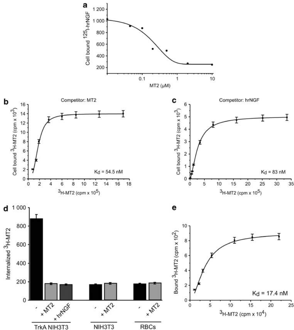
Figure 2 MT2 interactions with TrkA. (a) Displacement of 125 I-hrNGF bound to PC12 cells by MT2. PC12 cells were incubated with 0.1 nM 125 I-hrNGF in the presence or absence of different concentrations of MT2. Specific cell bound radioactivity was calculated and the results analyzed by Origin software. Results of one representative experiment out of three performed are shown. (b and c) Binding of 3 H-MT2 to TrkA NIH-3T3. NIH-3T3, stably transfected with full-length human TrkA, were incubated in triplicate with different concentrations of 3 H-MT2, in the presence or absence of excess cold MT2 (b) or 4 nM cold hrNGF (c). Specific cell bound radioactivity was calculated and the results analyzed by the Origin software (one-site binding assay). No specific binding was recorded on mock-transfected NIH-3T3 cells (not shown). (d) Internalization of 3 H-MT2. TrkA-NIH-3T3 or mock-transfected cells were incubated for 1 h at 4°C with 3 H-MT2 in the presence or absence of excess cold MT2 or hrNGF. Then, cells were washed and brought at 37°C for 1 h. Membrane radioactivity was eluted with 0.1 M glycine buffer, pH 2.8. RBC were incubated for 1 h at 37°C with 3 H-MT2 in the presence or absence of excess cold MT2 or hrNGF. Cells were lysed, and cell-bound radioactivity recorded. Data are expressed as mean bound radioactivity ± S.E. of triplicate cultures. Results of one representative experiments out of three performed are shown. (e) MT2 interaction with the ECD fraction of human recombinant TrkA. One microgram purified TrkA ECD was incubated in triplicate with different concentrations of 3 H-MT2, in the presence or absence of excess cold MT2. The mixture was absorbed on filter papers and, after washing, the radioactivity recorded. Data were analyzed by Origin software. Results from one representative experiments out of three performed are shown
